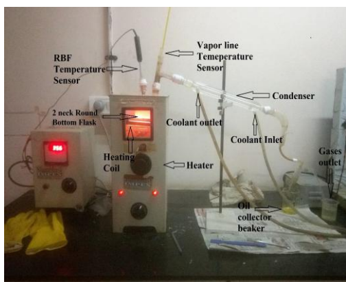
Fig. 1: Lab Scale Experimental Set-Up
