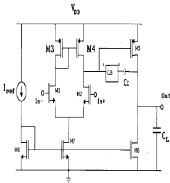
Figure2. The topology chosen for this Op-Amp design.
