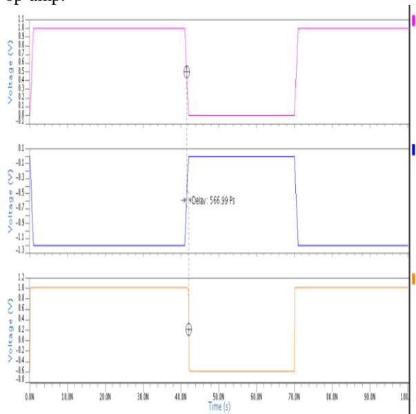
Figure 5. Result of Transient Analysis
