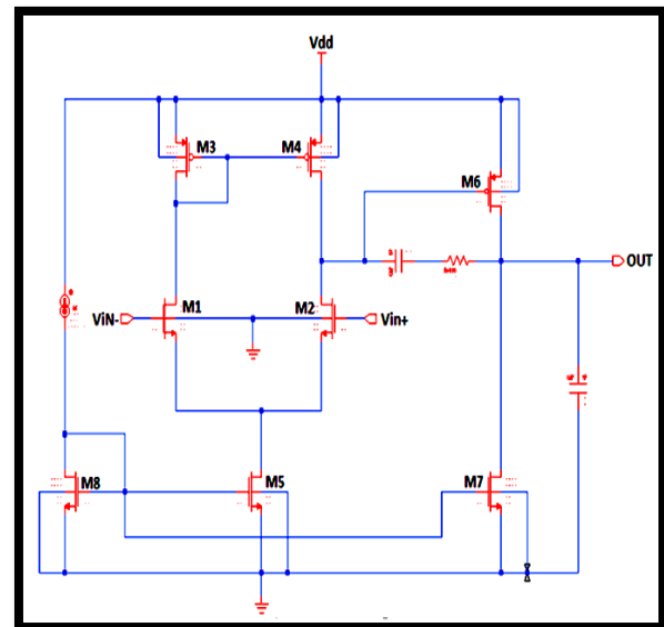
Figure 3. Schematic design of 2 stage CMOS Op-Amp
