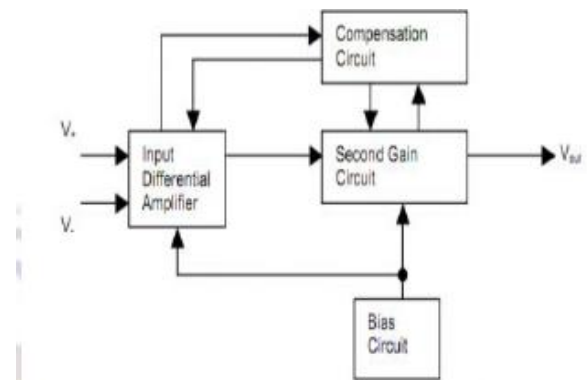
Figure 1. Block diagram of Op-Amp
