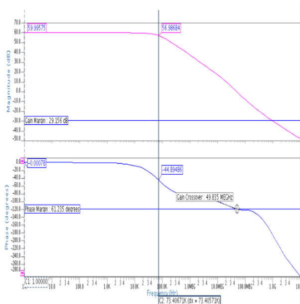
Figure 4. Output of AC Analysis
