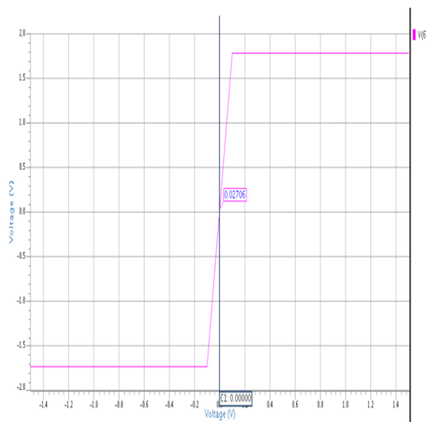
Figure 7. Output Offset
