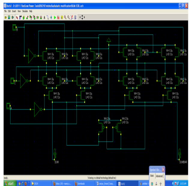
Figure6: ECR SUM Circuit
