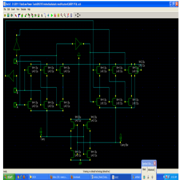
Figure5: PFAL Carry Circuit
