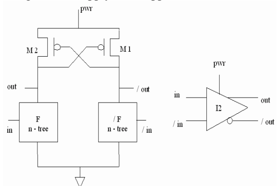
Figure1: The Basic Structure of the Adiabatic ECRL Logic.
