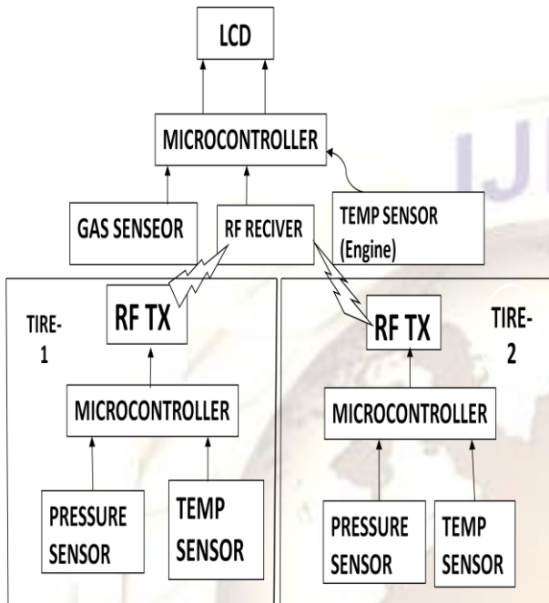
Figure 1: Block diagram of system
