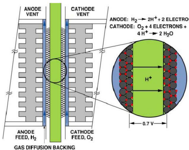
Fig. 3 Schematic of PEFC
