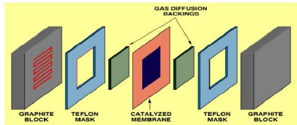
Fig.4 Single Structure of PEFC
