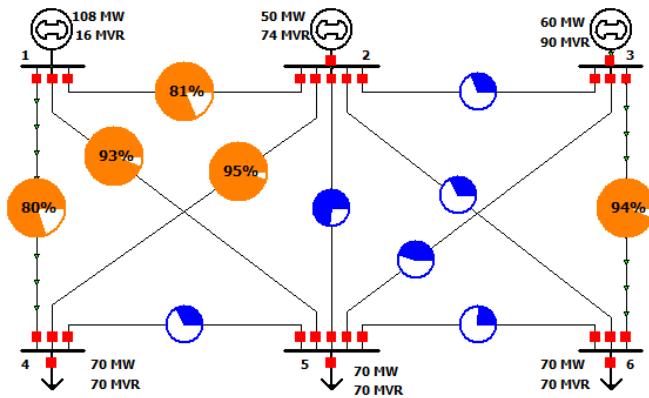
Fig. 3: IEEE 6bus System base case solution
