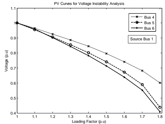
Fig. 4. PV Curves when Bus 1 is as a Source
