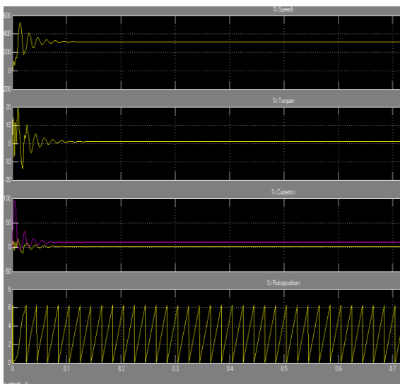
Fig 9 Simulink results
