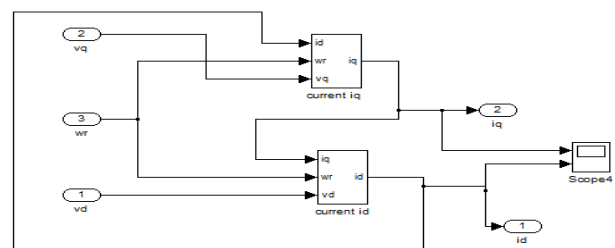
Fig.5. i_d, i_q current blocks
