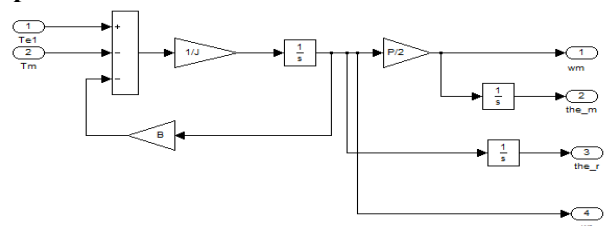
Fig.6. Speed model blocks
