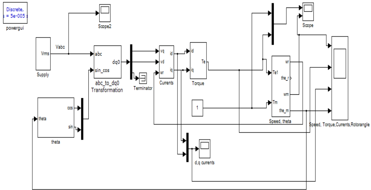
Fig 8. Simulink model of Permanent Magnet Synchronous Motor
