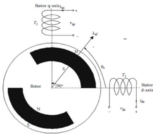
Fig.4. Dynamic model of PMSM
