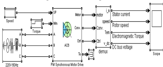
Fig. 2 matlab model for verifying characteristics
