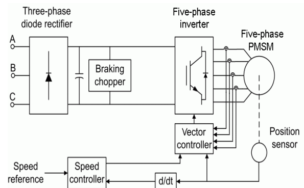
Fig 10. Proposed five phase PMSM modeled block diagram
