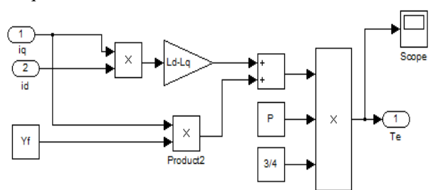
Fig.7. Torque model blocks of PMSM
