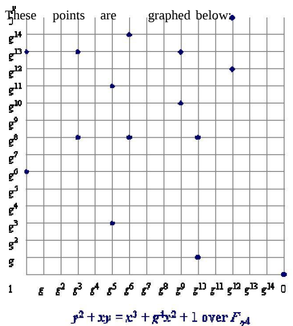
Figure1: Graph showing ECC Points
