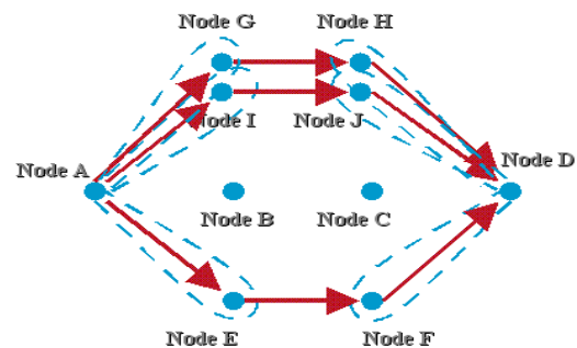
Fig. 4. Illustrates a single-source network with three routing paths.
