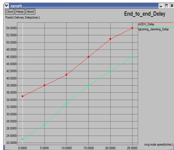
Graph2: end to end delay
