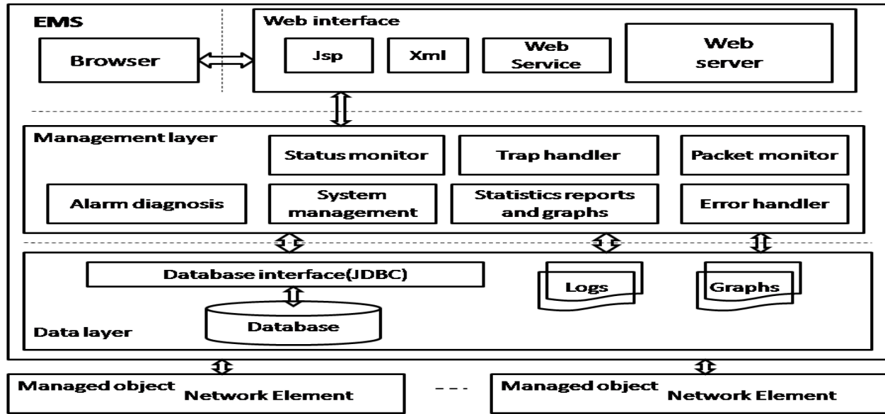
Figure 1. Structure of Element Management System
