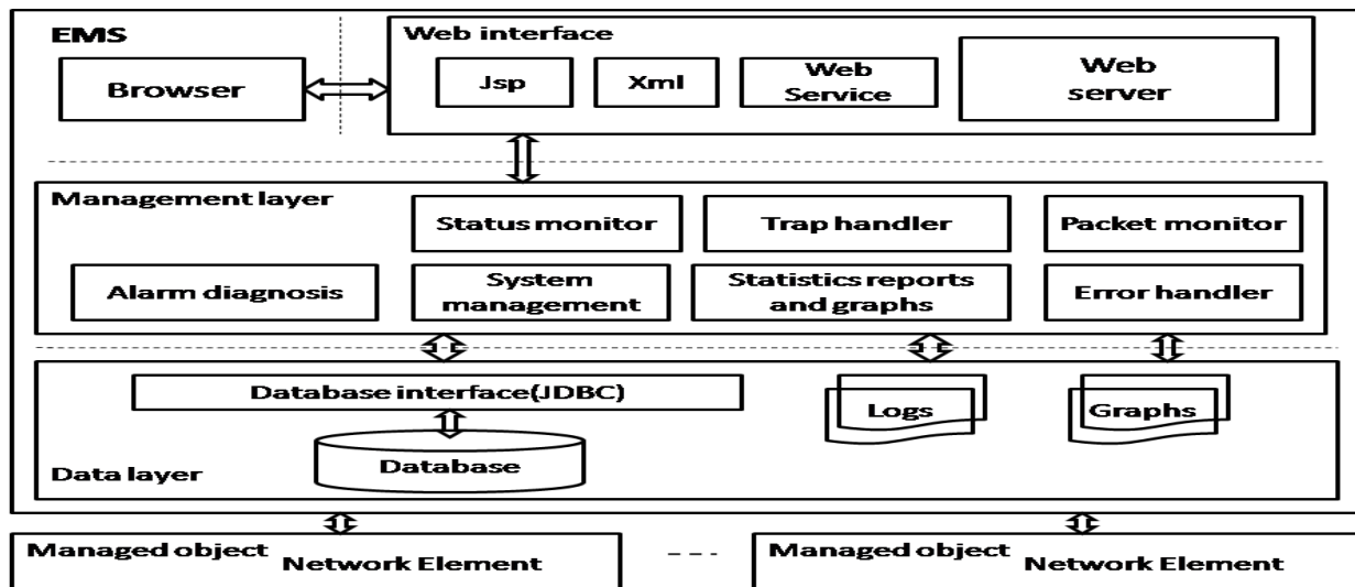
Figure 2. Technical architecture of EMS
