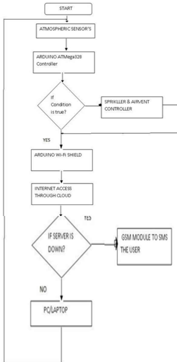
Fig 7: Flow chart
