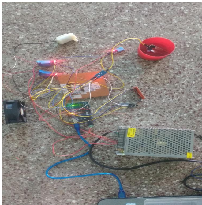
Fig 9: Hardware assembly
