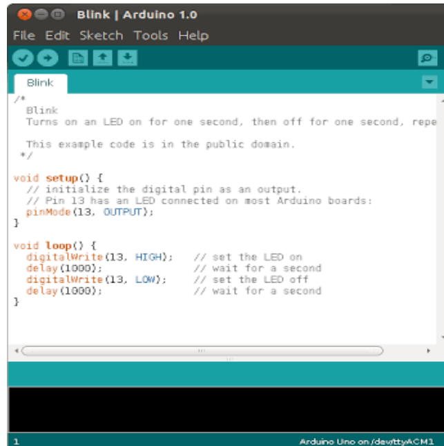
Fig 8: IDE Software
