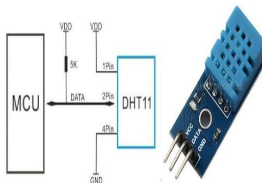
Fig 4: DHT11 Sensor
