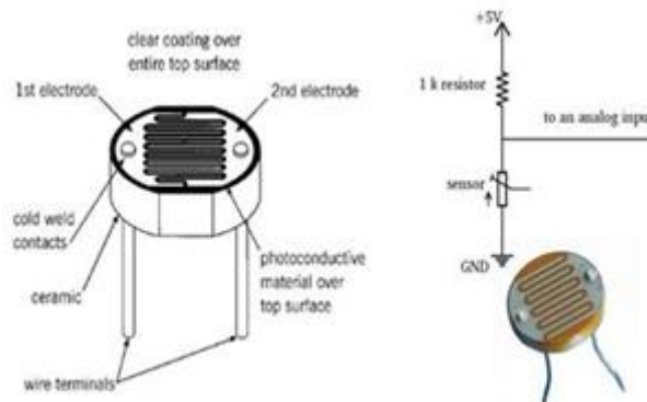
Fig 3: LDR Sensor
