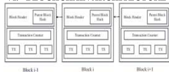
Fig 2: Block chain structure which contains continuous blocks[5].
