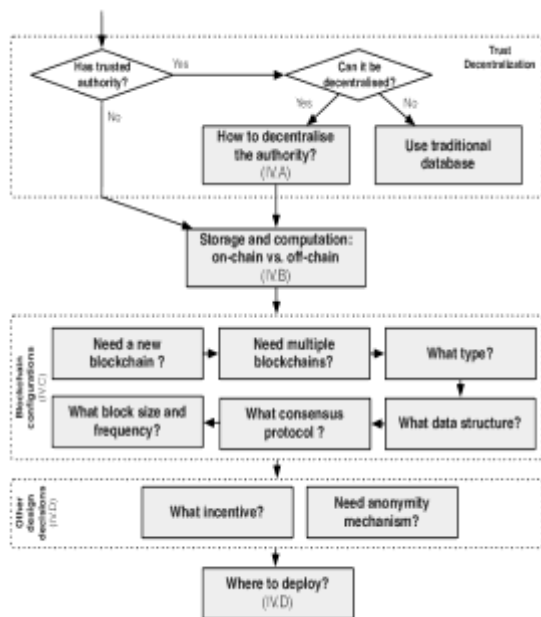
Fig 1: Design Process of Blockchain based applications
