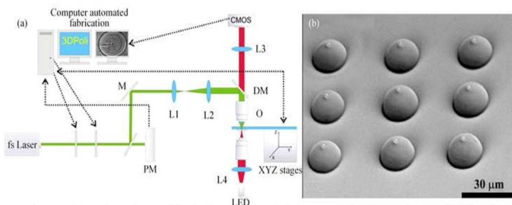
Figure 11. (a) Experimental setup and (b) microlenses fabricated using MPS. Reproduced from [63]. ©IOP Publishing Ltd. All rights reserved.
