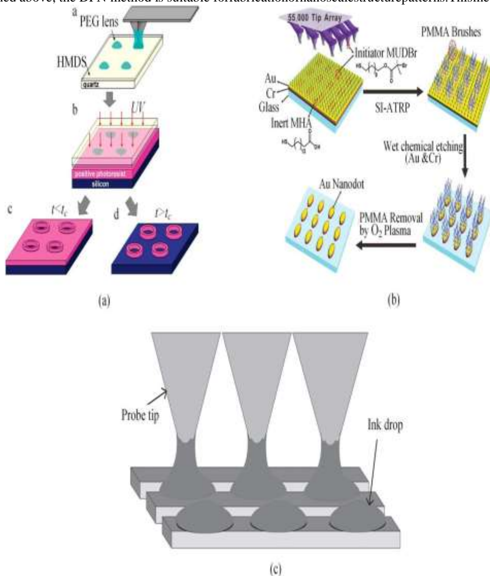
Figure 18. Schematic diagrams for some DPN processes. (a) DPN fabrication for polyethylene glycol (PEG) lens arrays on top of the hexamethylsilazane (HMDS)-coated quartz glass; subsequently, this array was used for ultraviolet photolithography. Reprinted with permission from [101]. Copyright (2010) American Chemical Society. (b) The DPN method was used to fabricate poly(methyl methacrylate) (PMMA) brushes on a gold surface to prepare for wet etching. [104] John Wiley & Sons. ©2017 WILEY-VCH Verlag GmbH & Co. KGaA, Weinheim. (c) DPN is used as a liquid ink to create dot patterns. [103] John Wiley & Sons. ©2018 WILEY-VCH Verlag GmbH & Co. KGaA, Weinheim.
