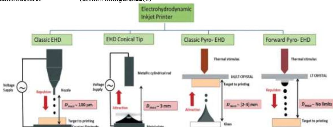
Figure 21. Schematic diagram of four different types of EHD jet printers. Reproduced from [106] with permission of The Royal Society of Chemistry.
