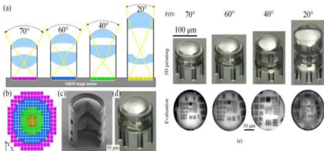
Figure 14. Three-dimensional-printed foveated imaging system. (a) Lenses with different focal lengths ( f=31, 38, 60, and 123 mm). (b) Pixelated image formed by the system. (c) Three-dimensional-printed doublet lens. (d) SEM image of the compound lens. (e) Printed lenses with different FOV (field of view) and corresponding imaging evaluation. Reprinted from [14]. © American Association for the Advancement of Science.
