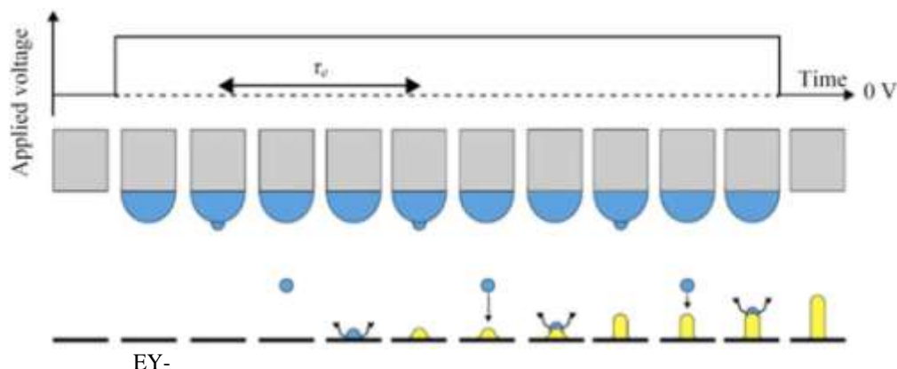
Figure 20. Schematic diagram of EHD jet printing. Reprinted with permission [102].
