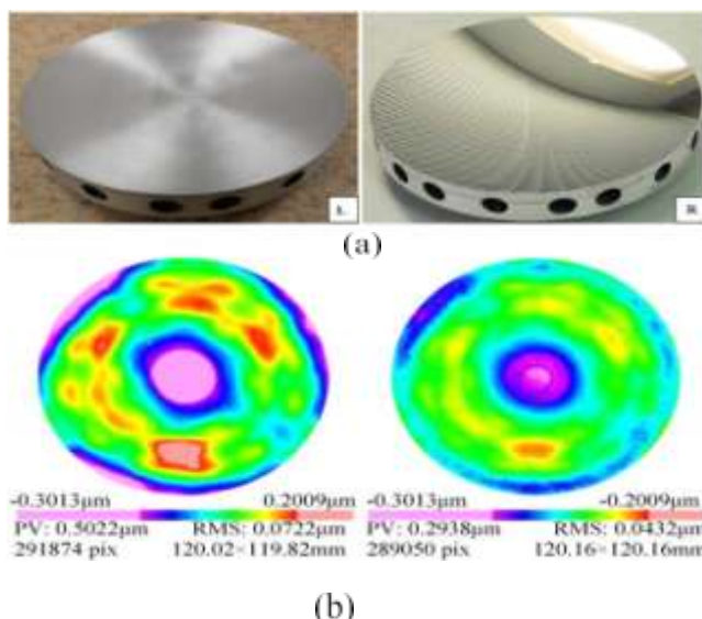
Figure 3. (a) A mirror manufactured by AM before post-processing (left) and after post-processing (right) and (b) surface roughness before (left) and after (right) the finishing process. Reprinted with permission from [31].
