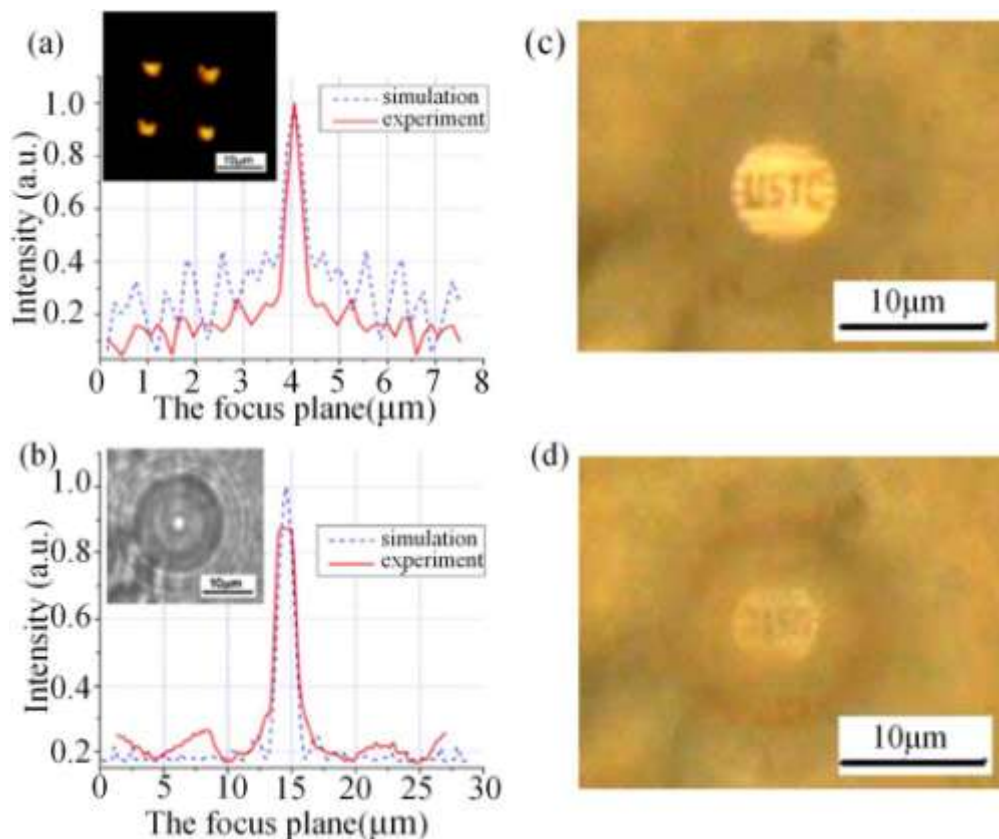
Figure 10. (a), (c) Optical performances of spherical microlenses and (b), (d) micro-Fresnel lenses fabricated by MPS. Reprinted with permission from [54], ©2006 Optical Society of America.
