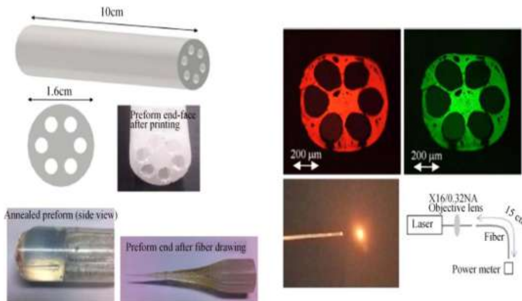
Figure 4. The printed optical fiber (left) and transmitted light with different wavelengths (wavelength = 630nm, 515nm, white light, and experimental setup) (right). Reprinted with permission from [39], ©2015 Optical Society of America.
