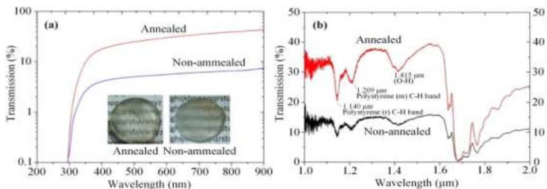
Figure 6. Transmission ranges of annealed and non-annealed fabricated fibers. (a) UV-visible spectra and (b) IR spectra. Reprinted with permission from [39], ©2015 Optical Society of America.
