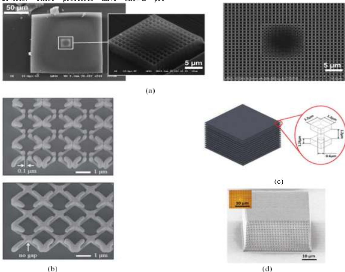
Figure 24. An example of DLW used in the fabrication of optical metamaterials. (a) SEM images of the metamaterial concentrator for a wavelength of 10.4 μm (left) and 5.6 μm (right). Reprinted by permission from Macmillan
