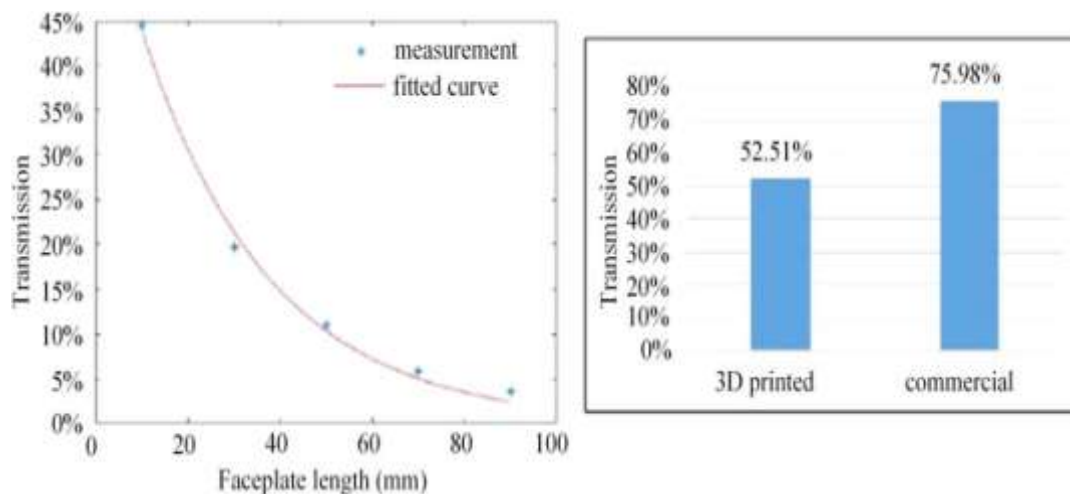
Figure 5. Transmission of the printed optical fibers. Reprinted with permission from [44], ©2018 Optical Society of America.
