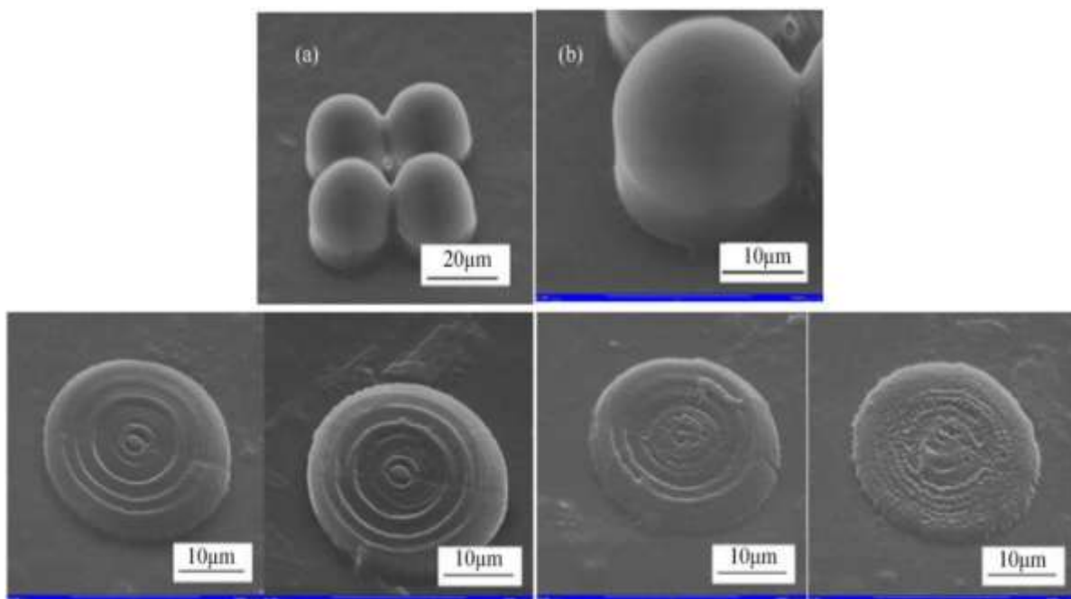
Figure 9. Images of the microlens fabricated in [54]. (a), (b) 2x2 microspherical lenses and a magnified view, micro-Fresnellens manufactured using several lateral scanning steps (bottom figures). Reprinted with permission from [54], ©2006 Optical Society of America.
