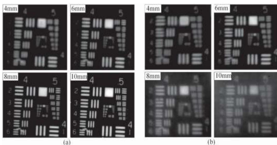
Figure 17. Resolution test of (a) a conventional lens and (b) a printed lens. Reprinted with permission from [100].
