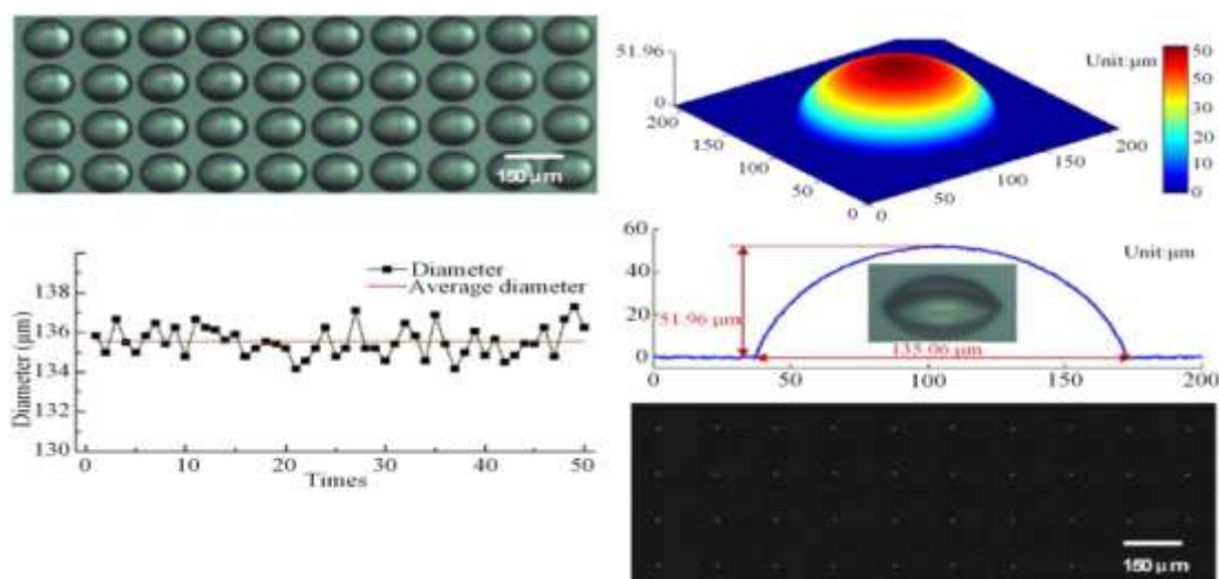
Figure 16. Microlens fabricated by DIW. Reprinted with permission from [99], ©2016 Optical Society of America.
