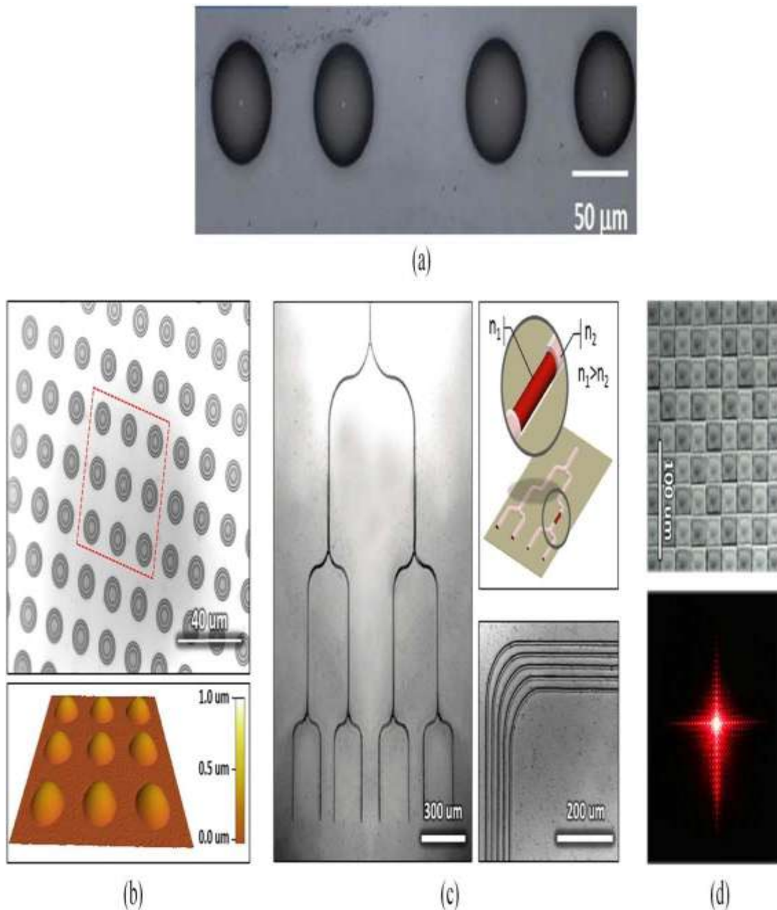
Figure 22. Some fabrication results of EHD jet printing. (a) PDMS microlens array fabricated by forward EHD jet printing. Reprinted with permission from [108]. (b) Optical microscope image and AFM image of microlens array. (c) Optical microscope image of EHD printed waveguides and illustration of a waveguide. (d) Image of EHD jet printed grating and the diffraction when a collimated laser beam passes through the grating. (b)–(d) Reprinted from [107], Copyright (2014), with permission from Elsevier.
