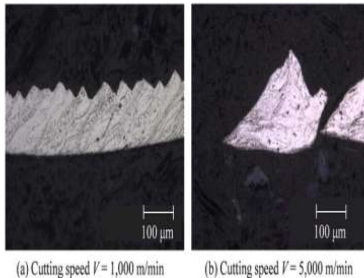
Figure 6. Chip morphologies of 7050-T7451 aluminum alloy with the uncut chip thickness of 0.1 mm and the cutting speeds (a) V = 1000 \text{ m min}^{-1} and (b) V = 5000 \text{ m min}^{-1} , respectively. Reproduced with permission from [79].
