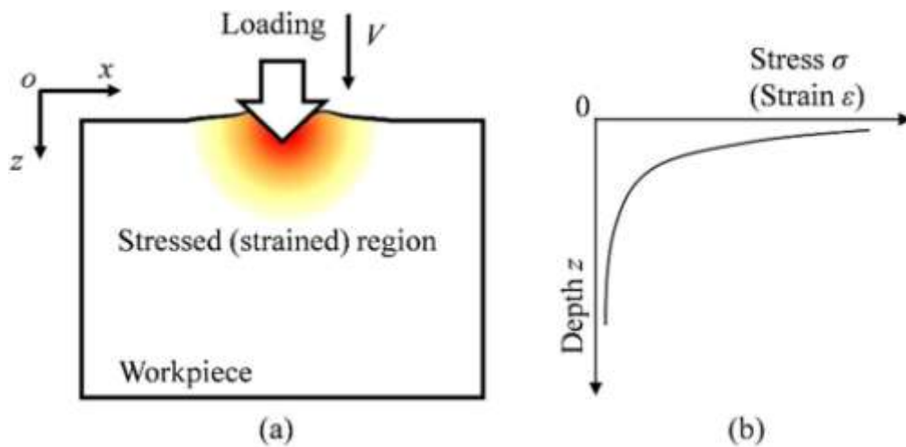
Figure 9. Schematics of (a) a stressed (strained) region around the loading point; (b) stress (strain) distribution
