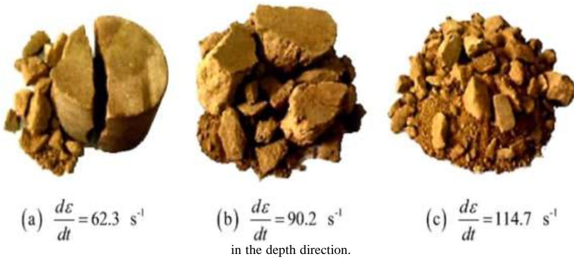
Figure 10. Fragments of sandstone impacted at different strain rates. Reproduced with permission from [102].
