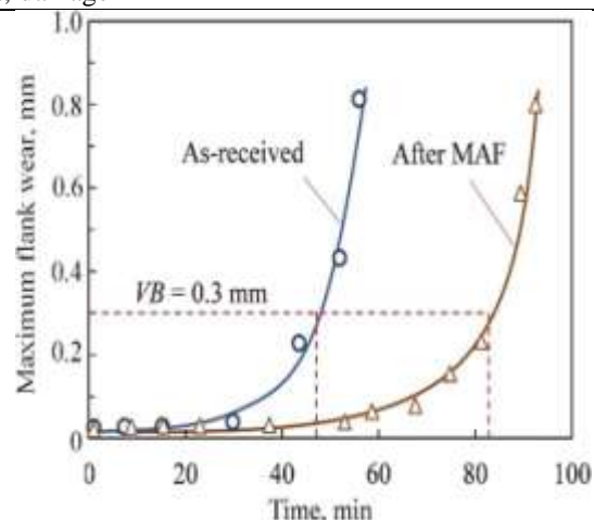
Figure 1. Maximum flank wear of the different tool inserts versus machining time (cutting speed: 100 \text{ m min}^{-1} , feed: 75 \text{ }\mu\text{m/rev} , depth of cut: 1.0 \text{ mm} , coolant: 5% vol. trim solution). Reprinted from [23], Copyright (2012), with permission from Elsevier.
