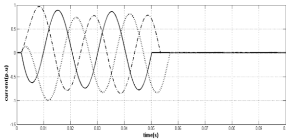
Fig. 7. Fault current (in pu) with IBDG (time in sec)
