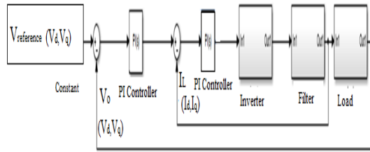
Fig. 2. Dual loop voltage regulator [18]
