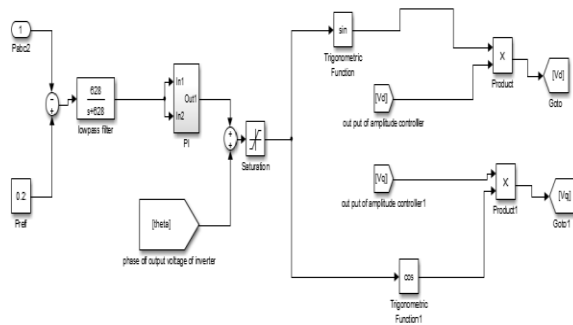
Fig. 3. Phase controller for grid synchronization and constant active power
