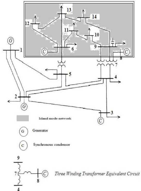
Fig. 4. One Line Diagram of IEEE-14 Bus System [22]
