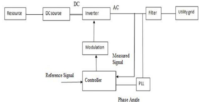
Fig. 1. Modelling of inverter based DG[15]
