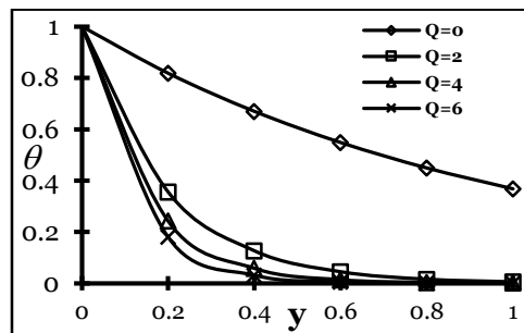
Fig. 4 (iii): Temperature for Q
