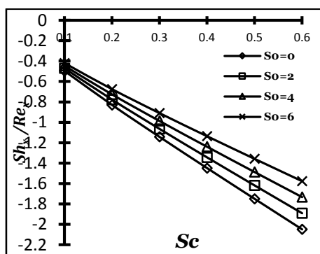
Fig. 4 (viii): Sherwood number for Sc and So
