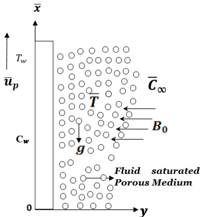
Figure 2(a): Physical model and coordinate system
