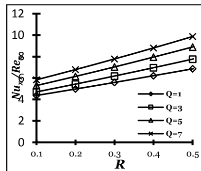
Fig. 4 (x): Nusselt number for R and Q
