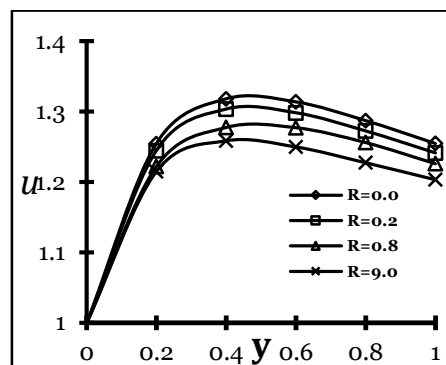
Fig. 4 (iv): Velocity distribution on R
