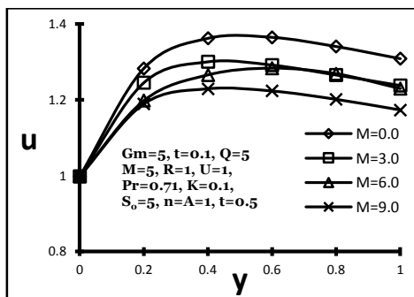
Fig. 4 (i): Velocity distribution on M
