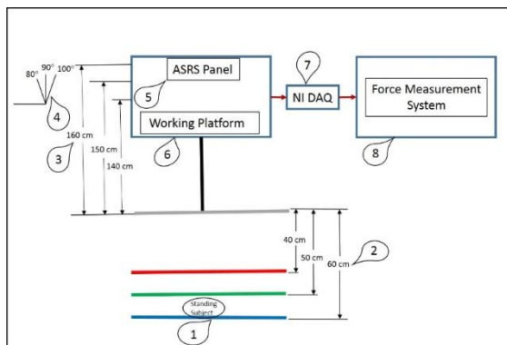
Fig. 3. Schematic diagram of the experimental set-up for experimental investigations
