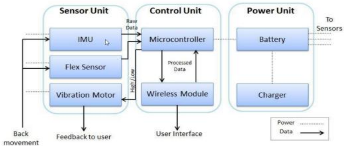
Fig 4 : Block Diagram of Smart wearable posture detection and alert system
