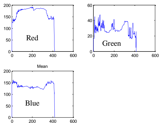
Fig. 3 (b) Analysis of Thermal Image of Healthy bearing Induction Motor
