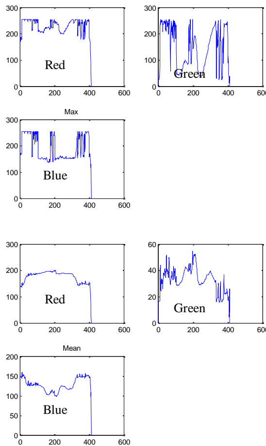
Fig. 4 (b) Analysis of Thermal Image of Bearing fault (defected Ball) of Induction Motor after 5 min. run
