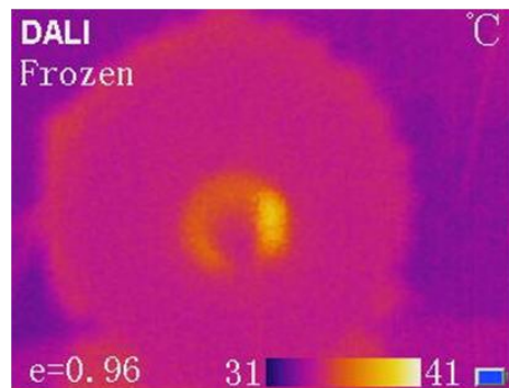
Fig. 4 (a) Bearing fault (defected Ball) of Induction Motor after 5 min. run
