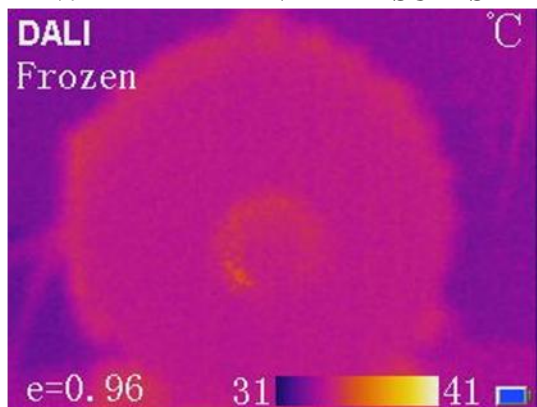
Fig. 3 (a) Thermal Image of Healthy bearing Induction Motor
