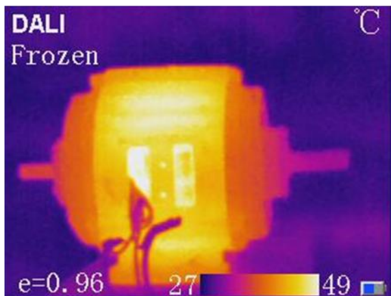
Fig. 7 (a) Healthy Induction Motor - front view
