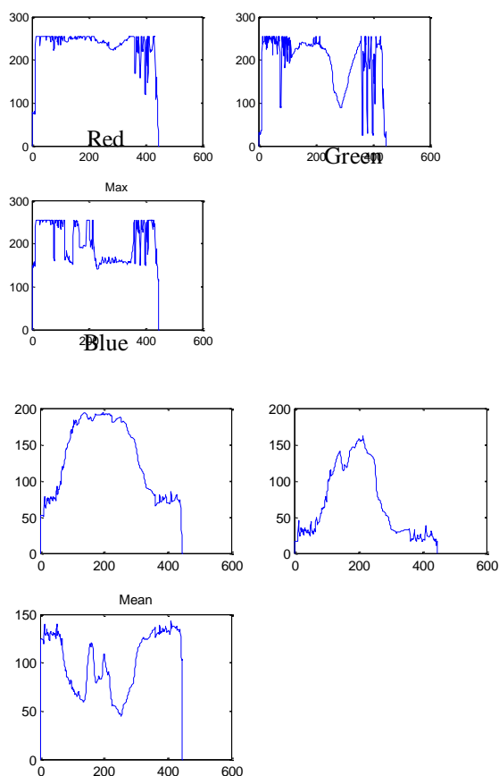
Fig. 7 (b) Image analysis of Healthy Induction Motor - front view
