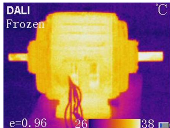
Fig. 6 (a) Faulty Induction Motor - front view
