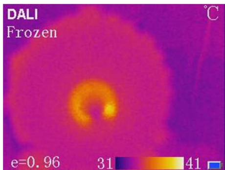
Fig. 5 (a) Bearing fault (defected Ball) of Induction Motor after 10 min. run
