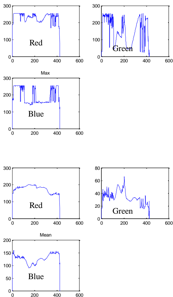
Fig. 5 (b) Analysis of Thermal Image of Bearing fault (defected Ball) of Induction Motor after 10 min. run
