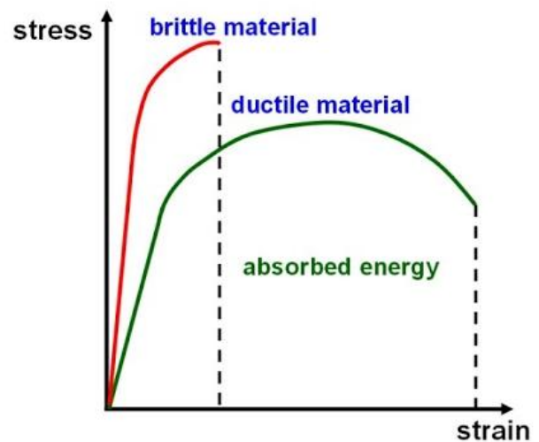
Label 1.7 depicts the fracture toughness difference between brittle and ductile materials.
