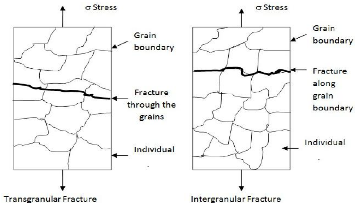
Label 1.2 illustrates the two types of brittle fractures.
