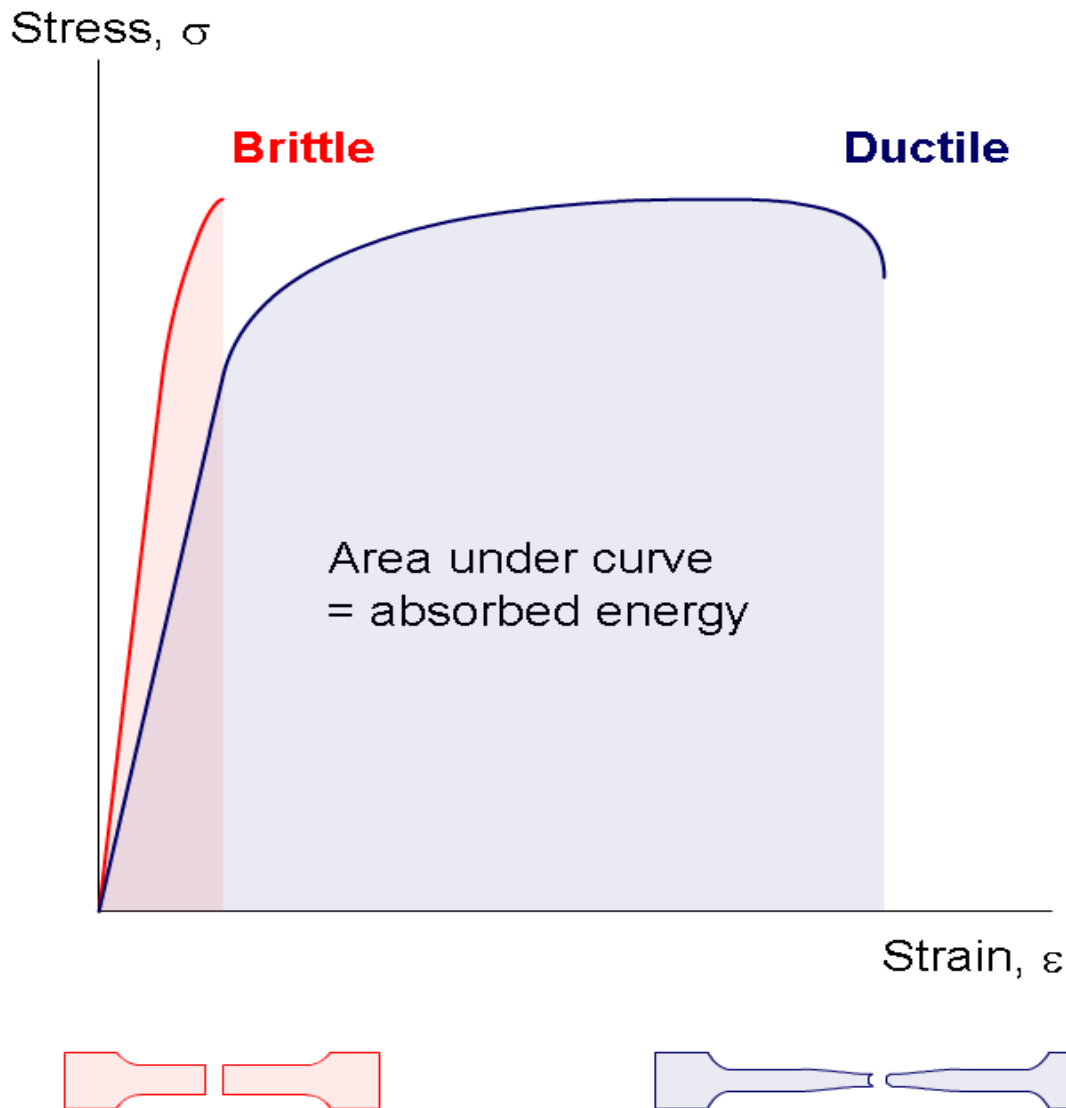
Label 1.8 illustrates the absorbed energy observed when both the brittle and ductile materials are under a certain amount of stress.
