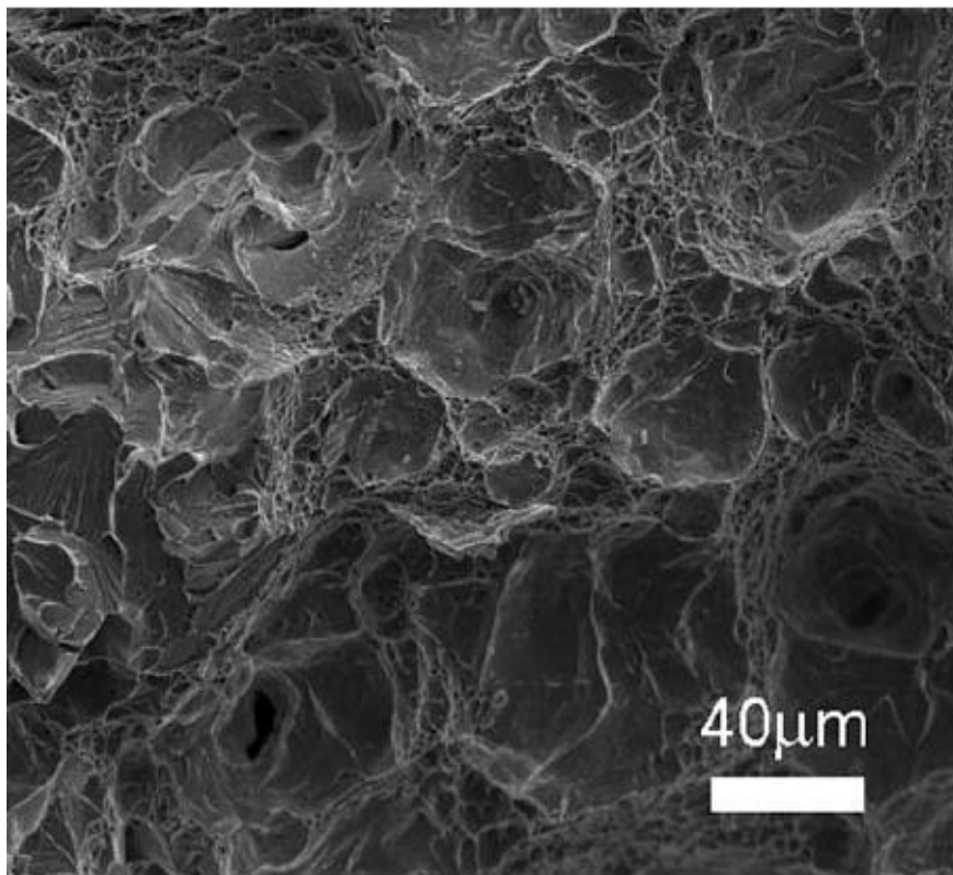
Label 1.5 illustrates the SEM micrograph of ductile fracture due to transformation toughening for prototype tempered at 575 ° C for five hours.
