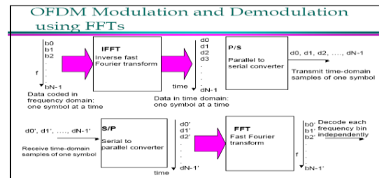
FIGURE 3. Modulation and Demodulation in OFDM
