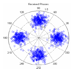
FIGURE 7. OFDM received signals Plots.
