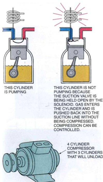
Figure 27-10 Capacity control for a compressor.
