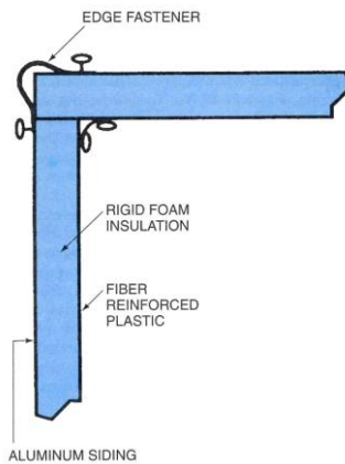
Figure 27-18 Sandwich construction for truck walls.
