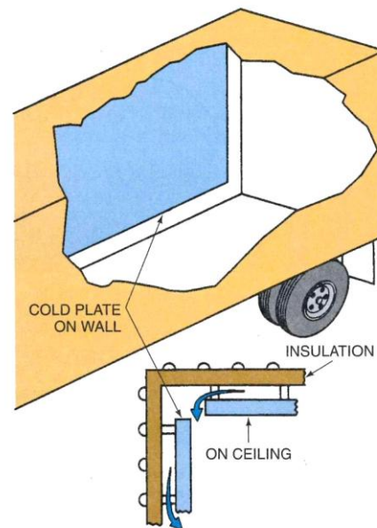
Figure 27-5 Cold plates mounted in a truck body.
