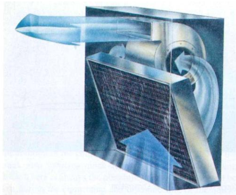
Figure 27-12 Evaporator for a nose-mount refrigeration unit.
