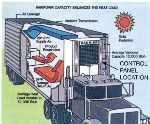
Figure 27-13 Air distribution system for truck. Reproduced courtesy of Carrier Corporation
