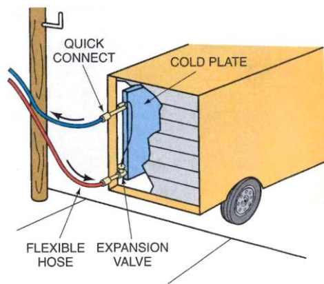
Figure 27-6 Cold plate connected to the refrigeration system at the dock.
