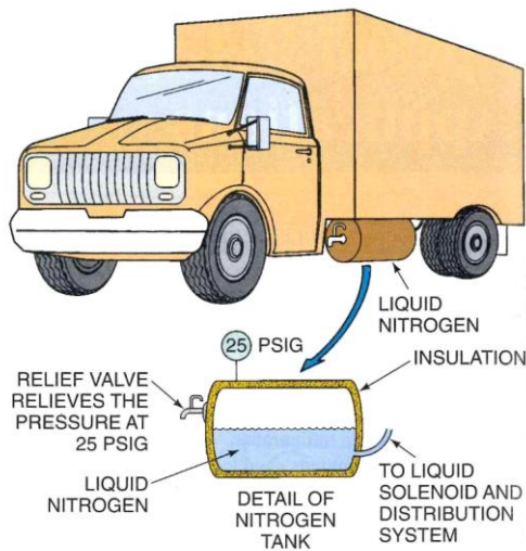
Figure 27-3 Nitrogen cylinder maintained at about 25 psig.
