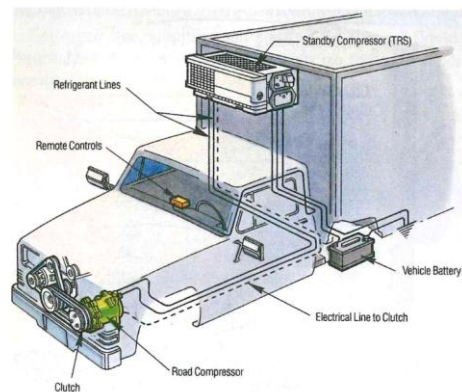
Figure 27-7 This truck refrigeration is driven from the truck's engine and may be cycled by means of an electric clutch. Reproduced courtesy of Carrier Corporation
