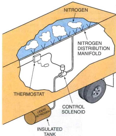
Figure 27-4 Control for a liquid nitrogen cooling system.
