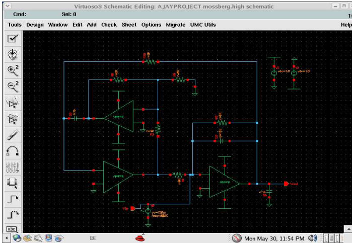
Figure 5.1 Schematic of Ackerberg-Mossberg high pass filter
