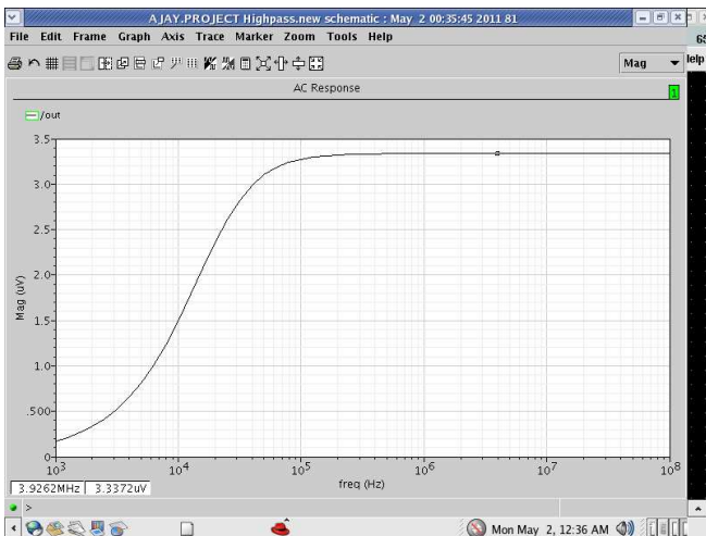
Figure 5.2 AC Response of Ackerberg –Mossberg high pass filter:
