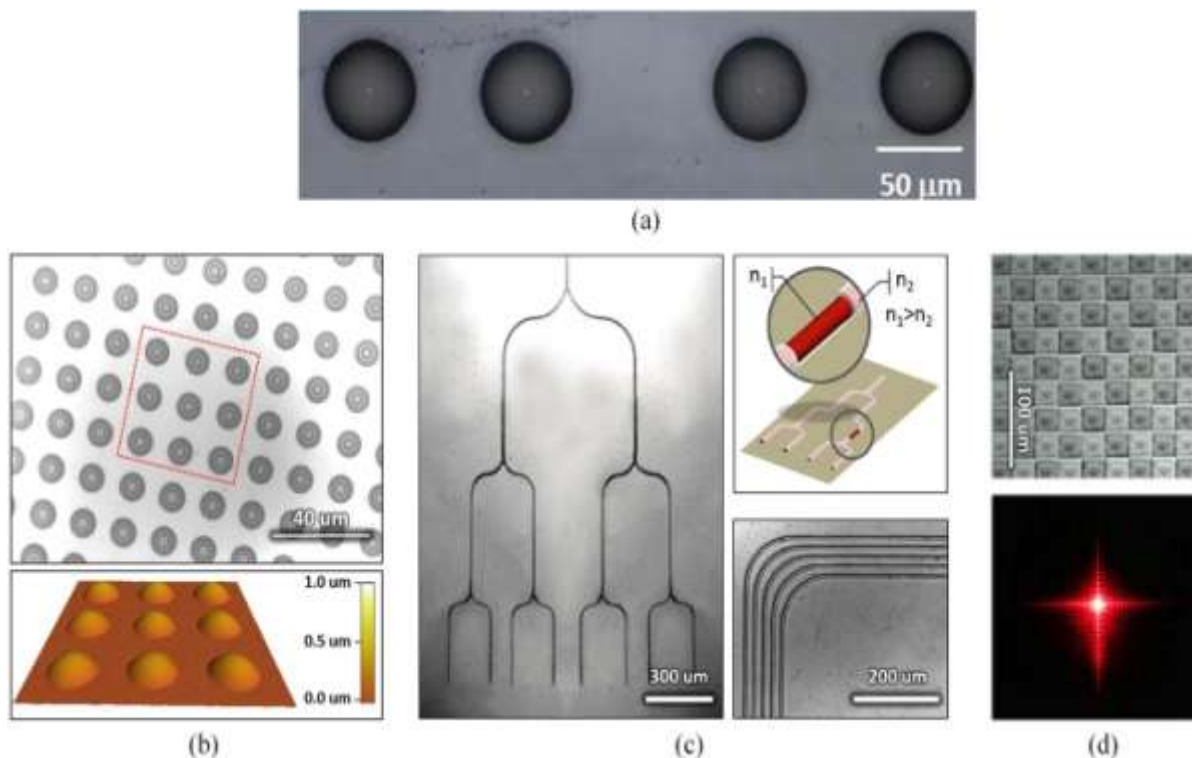
Figure 22. Some fabrication results of EHD jet printing. (a) PDMS microlens array fabricated by forward EHD jet printing. Reprinted with permission from [108]. (b) Optical microscope image and AFM image of microlens array. (c) Optical microscope image of EHD printed waveguides and illustration of a waveguide. (d) Image of EHD jet printed grating and the diffraction when a collimated laser beam passes through the grating. (b)–(d) Reprinted from [107], Copyright (2014), with permission from Elsevier. material to fabricate a microlens array [108]. The fabrication results are shown in figure 22(a).
