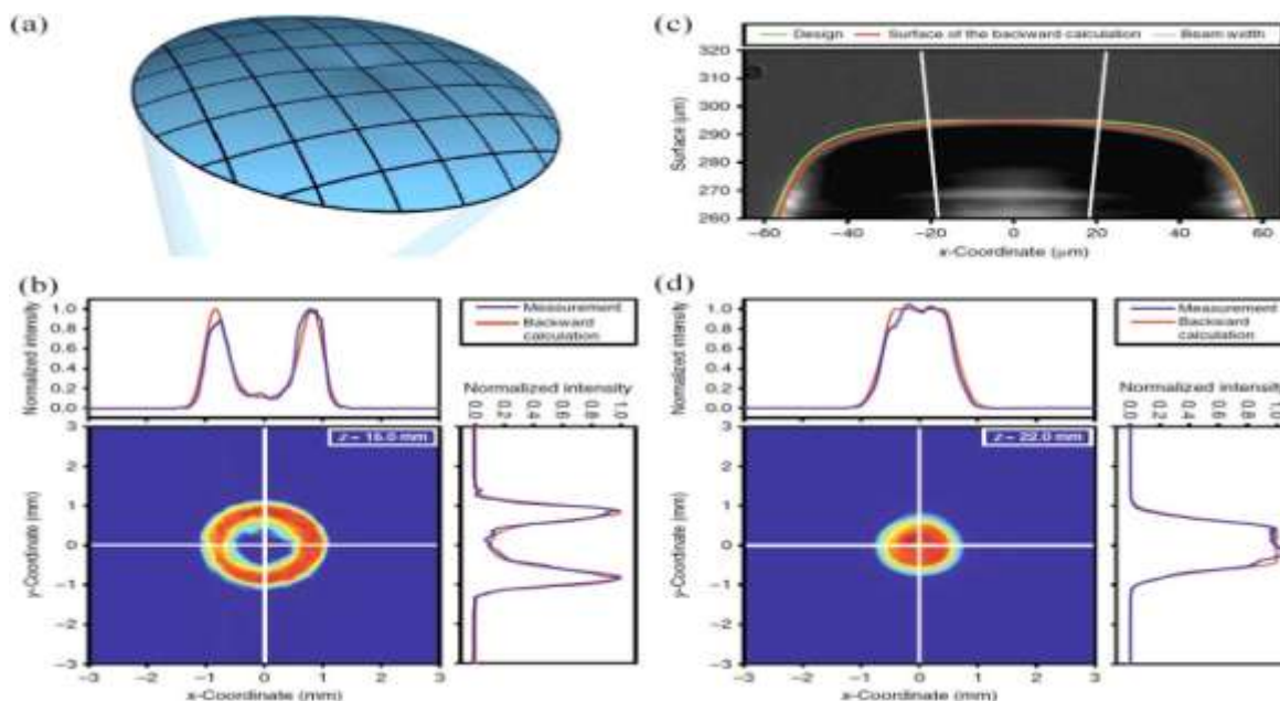
Figure 15. (a) Donut-shaped optical surface on an optical fiber, (b) Corresponding experimental result of a donut-shaped surface, (c) hat-shaped optical surface on the fiber, and (d) corresponding experimental result of hat-shaped surface. Reprinted by permission from Macmillan Publishers Ltd: Nature Communications [82], Copyright (2016).
