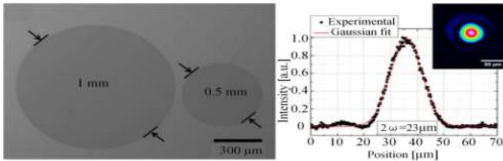
Figure 13. A lens on the scale of millimeters and its corresponding performance graph [64].
