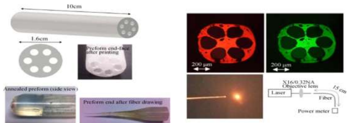
Figure 4. The printed optical fiber (left) and transmitted light with different wavelengths (wavelength = 630 nm, 515 nm, white light, and experimental setup) (right). Reprinted with permission from [39], © 2015 Optical Society of America.
