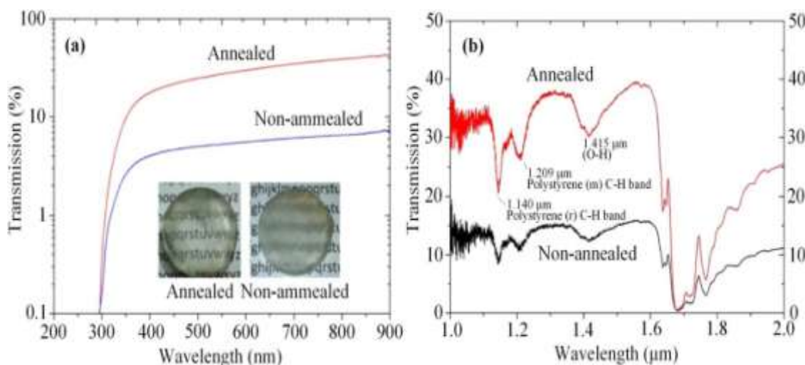
Figure 6. Transmission ranges of annealed and non-annealed fabricated fibers. (a) UV-visible spectra and (b) IR spectra. Reprinted with permission from [39], © 2015 Optical Society of America.
