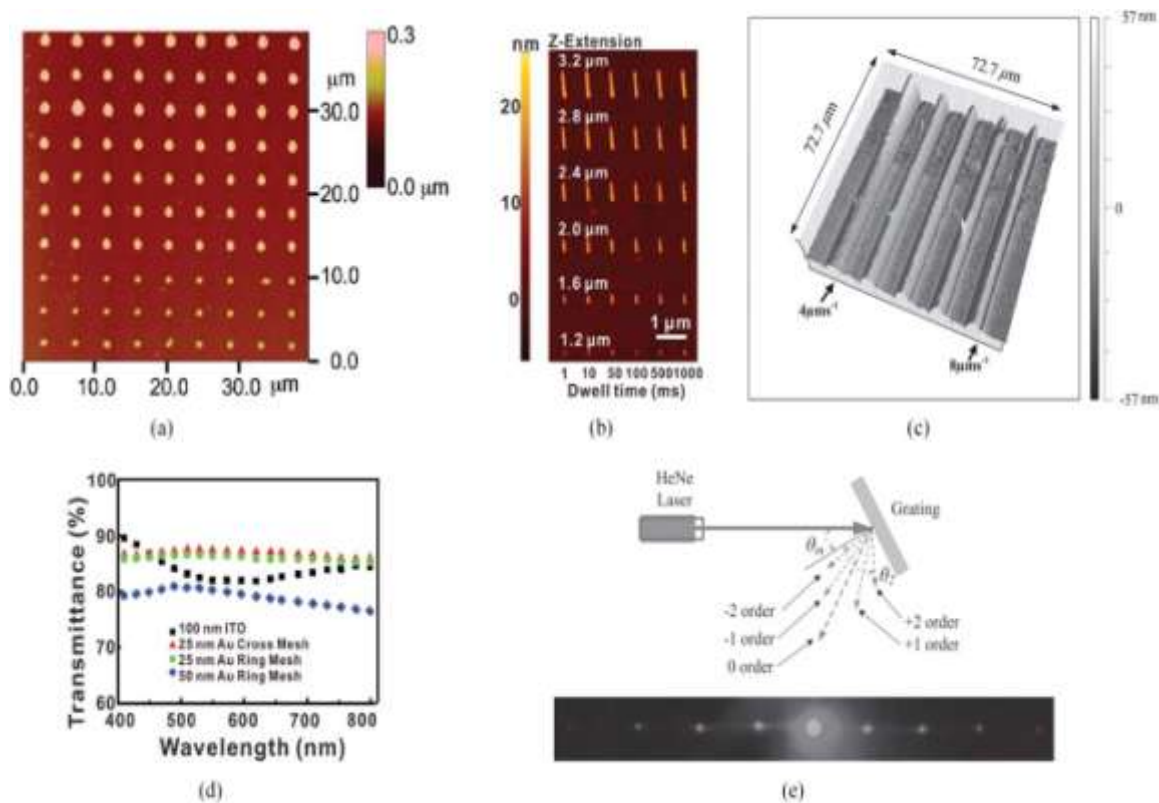
Figure 19. Fabrication results of DPN. (a) Atomic force microscopic (AFM) image of the PEG nanoscale lens arrays generated by DPN. The different size of each row is attributed to different substrate dwell times. Reprinted with permission from [101]. Copyright (2010) American Chemical Society. (b) AFM image of PMMA brushes preparing for wet etching fabrication by DPN. [104] John Wiley & Sons. © 2017 WILEY-VCH Verlag GmbH & Co. KGaA, Weinheim. (c) AFM image of the grating pattern array; different lines are fabricated by different tip velocities. John Wiley & Sons. © 2017 WILEY-VCH Verlag GmbH & Co. KGaA, Weinheim. (d) Transmission rate of the incident light with different wavelengths on the substrate with or without gold nanoscale patterns. [104] John Wiley & Sons. © 2017 WILEY-VCH Verlag GmbH & Co. KGaA, Weinheim. (e) Experimental device used to measure diffraction orders and the diffractive spectrum of the grating fabricated by DPN. [103] John Wiley & Sons. © 2017 WILEY-VCH Verlag GmbH & Co. KGaA, Weinheim.
