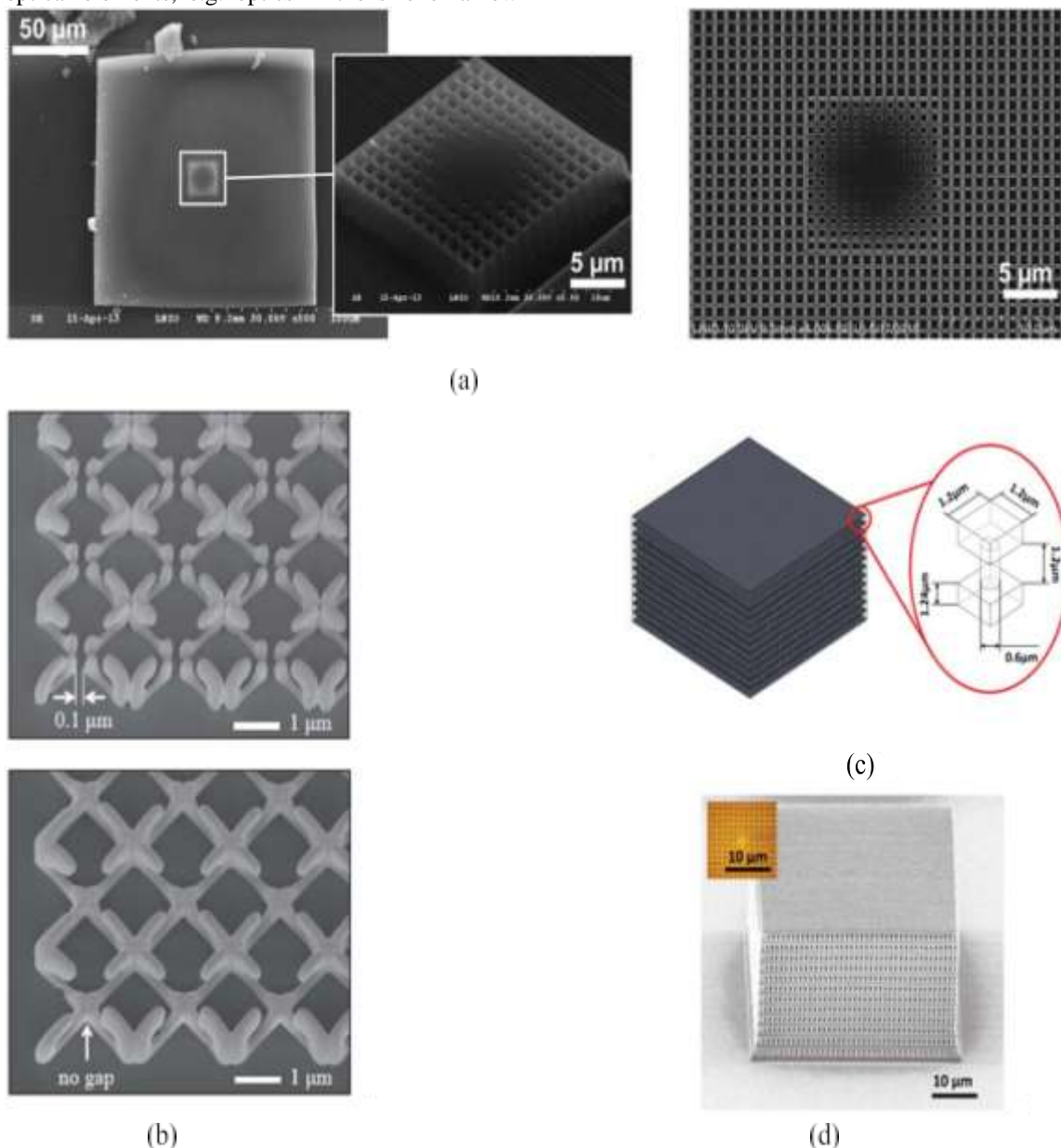
Figure 24. An example of DLW used in the fabrication of optical metamaterials. (a) SEM images of the metamaterial concentrator for a wavelength of 10.4 \mu\text{m} (left) and 5.6 \mu\text{m} (right). Reprinted by permission from Macmillan Publishers Ltd: Scientific Reports [115], Copyright (2016). (b) SEM image of vertical split-ring
