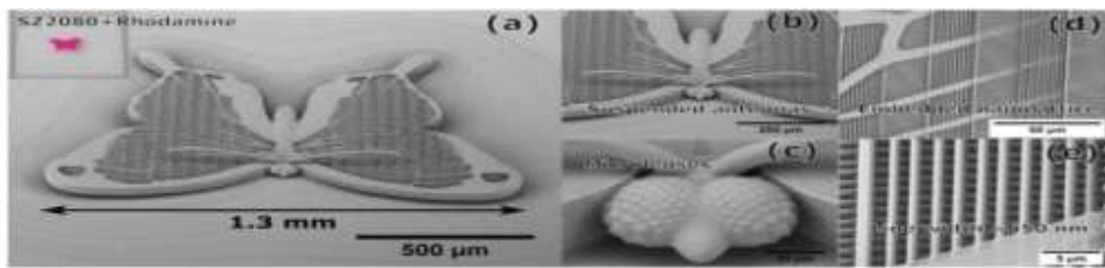
Figure 12. (a) Scanning electron microscope (SEM) image of the whole structure. (b) Enlarged view of the antennae. (c) Close-up view of the microlenses on the head, and (d) embedded nanolattice of a wing [64].
