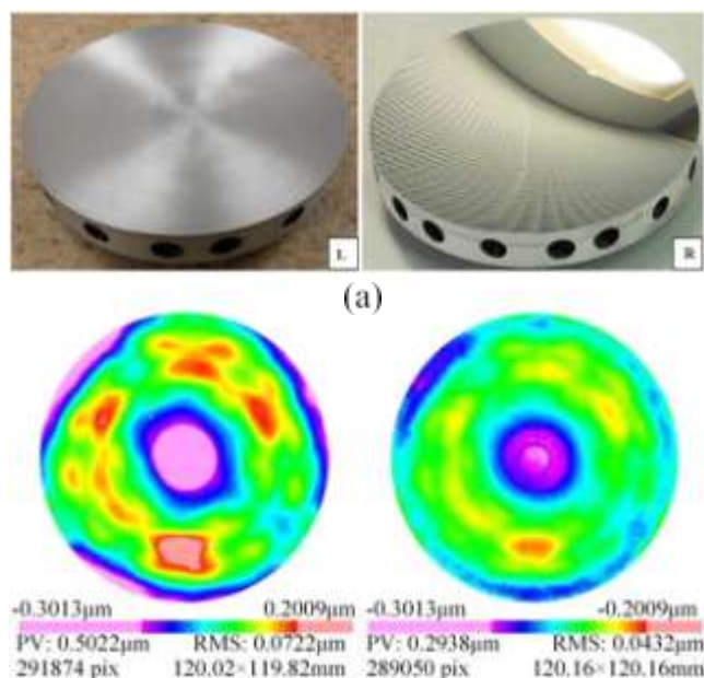
Figure 3. (a) A mirror manufactured by AM before post-processing (left) and after post-processing (right) and (b) surface roughness before (left) and after (right) the finishing process. Reprinted with permission from [31].
