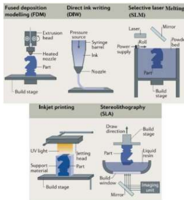
Figure 1. Popular additive manufacturing methods. Reprinted by permission from Macmillan Publishers Ltd: Nature Reviews Materials [30], Copyright (2018).
