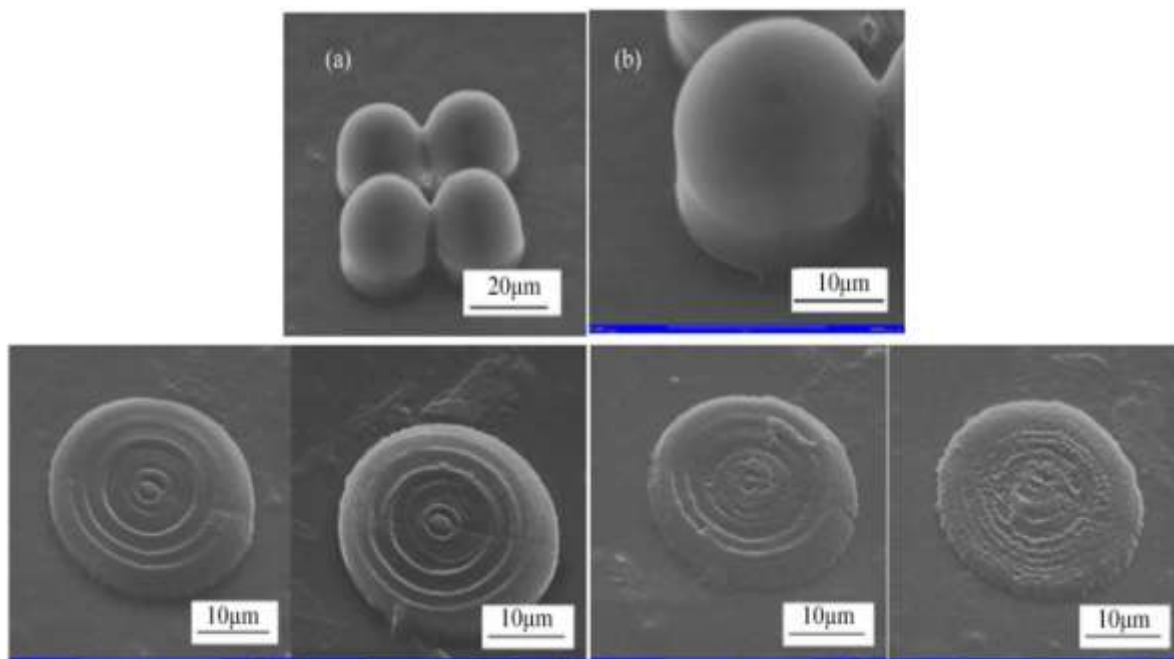
Figure 9. Images of the microlens fabricated in [54]. (a), (b) 2 \times 2 microspherical lenses and a magnified view, micro-Fresnel lens manufactured using several lateral scanning steps (bottom figures). Reprinted with permission from [54], © 2006 Optical Society of America.
