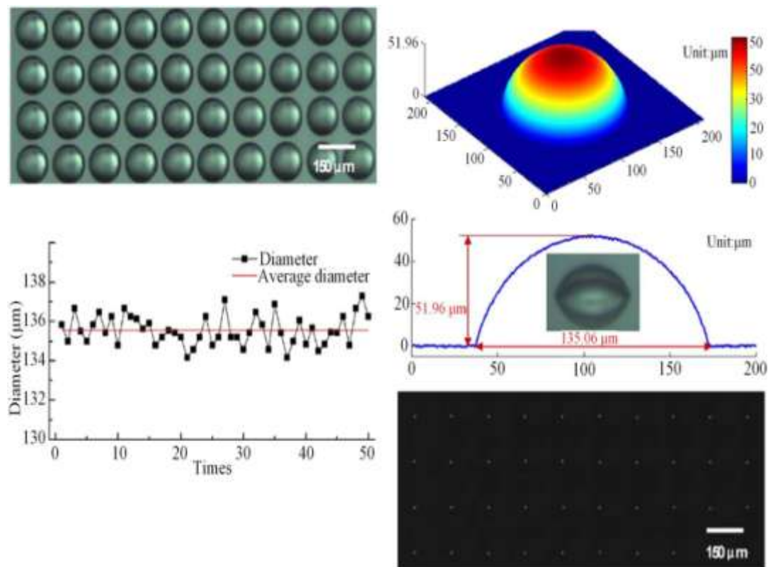
Figure 16. Microlens fabricated by DIW. Reprinted with permission from [99], © 2016 Optical Society of America.
