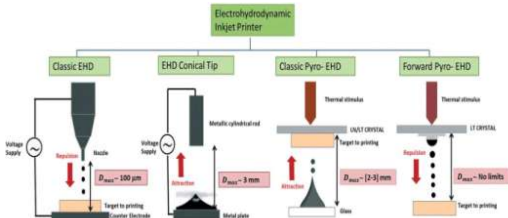
Figure 21. Schematic diagram of four different types of EHD jet printers. Reproduced from [106] with permission of The Royal Society of Chemistry.
