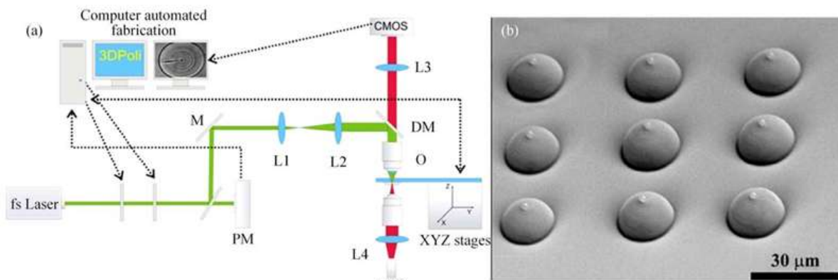
Figure 11. (a) Experimental setup and (b) microlenses fabricated using MPS. Reproduced from [63]. © IOP Publishing Ltd. All rights reserved.
