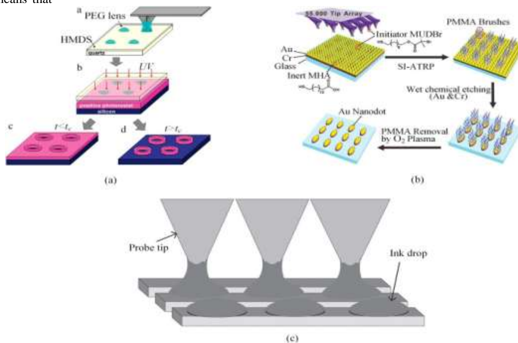
Figure 18. Schematic diagrams for some DPN processes. (a) DPN fabrication for polyethyleneglycol (PEG) lens arrays on top of the hexamethyldisilazane (HMDS)-coated quartz glass; subsequently, this array was used for ultraviolet photolithography. Reprinted with permission from [101]. Copyright (2010) American Chemical Society. (b) The DPN method was used to fabricate polymethylmethacrylate (PMMA) brushes on a gold surface to prepare for wet etching. [104] John Wiley & Sons. © 2017 WILEY-VCH Verlag GmbH & Co. KGaA, Weinheim. (c) DPN is used as liquid ink to create dot patterns. [103] John Wiley & Sons. © 2018 WILEY-VCH Verlag GmbH & Co. KGaA, Weinheim.
