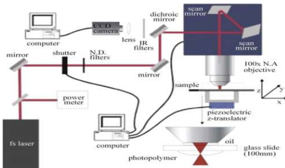
Figure 23. Schematic diagram of a typical DLW experiment system. Reprinted from [109], Copyright (2015), with permission from Elsevier.
