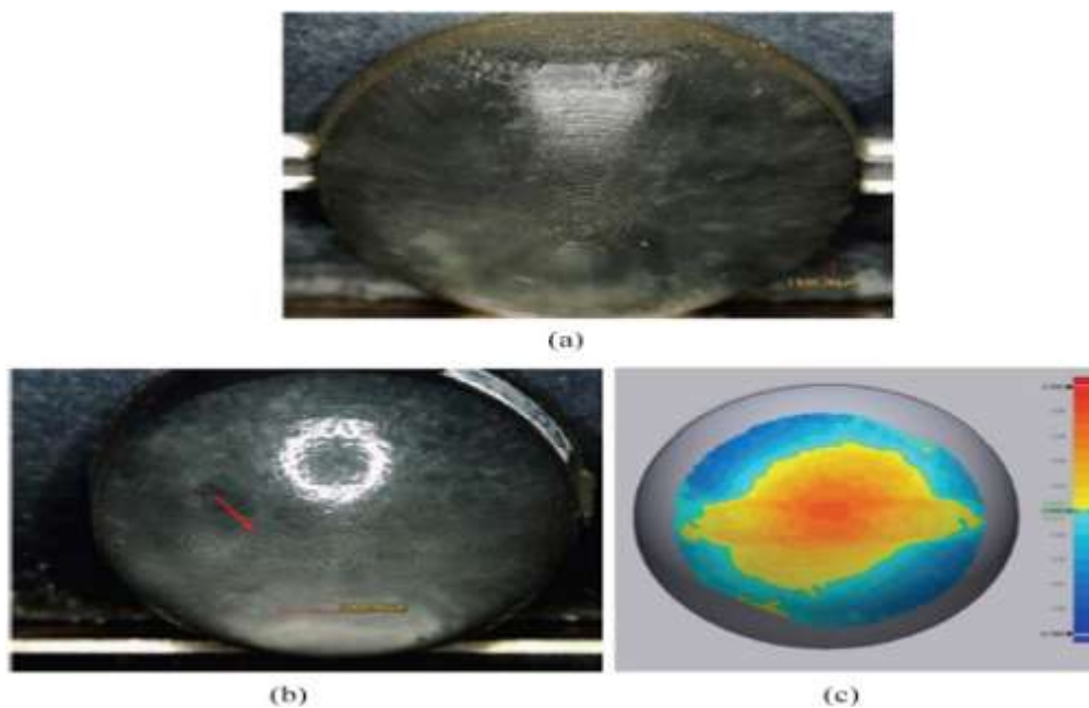
Figure 8. (a) A lens manufactured by SLA, (b) step profile, and (c) shape deviation. Reprinted with permission from [20].
