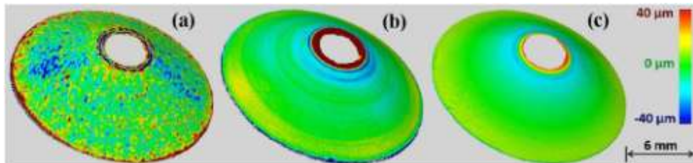
Figure 2. Additively manufactured conic mirror assessment. (a) SLM printed part (b) after grinding and (c) after polishing. Reprinted with permission from [29].
