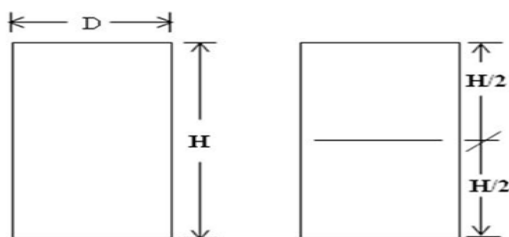
Fig.4.1. 100 Mm Diameter (D) And 200 Mm Height (H) Soil Samples With Geotextile Reinforcing Layer Configuration.
