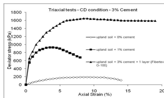
Fig. 3. Stress-Strain Curves Of Reinforced And 3% Cement Modified Marginal Soil Under Drained Condition At 7 Days Curing For \sigma_3 = 150 Kpa.
