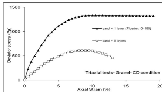
Fig.4. Stress-Strain Curves From Triaxial Tests On Reinforced Gravel Under Drained Condition.
