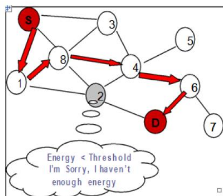
Figure 2.b: Route established with E-AODV
