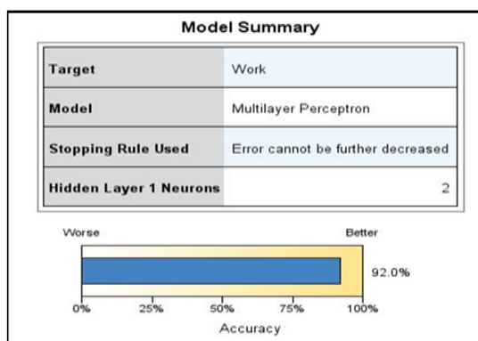
Fig. 5. Classification accuracy
