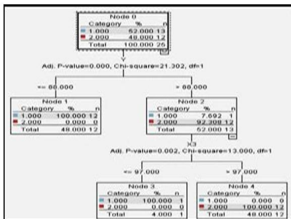
Fig. 6. Analyses of Decision Tree Model “by the authors”
