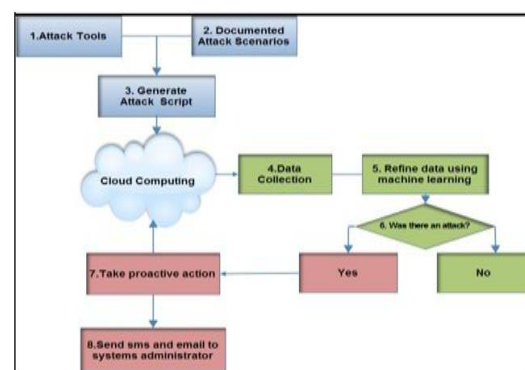
Fig. 4. Attack detection and proactive resolution in single cloud environment Using machine learning (modified by the authors) [8]
