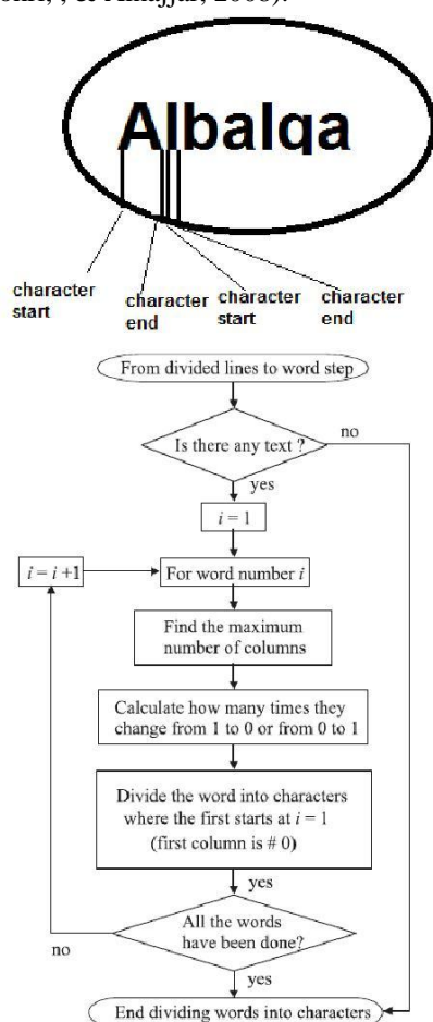
Figure 6. Character segmentation
