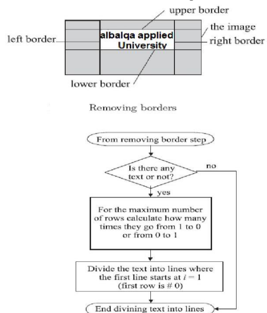
Figure 5. Converting Text into Lines
