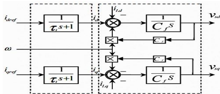
Fig. 5. Block diagram of dynamic load model with inverter model
