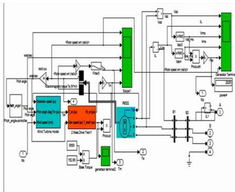
Fig 8 MATLAB Model of Wind generation circuit.
