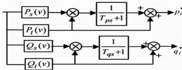
Fig. 4. Dynamic load model for power references
