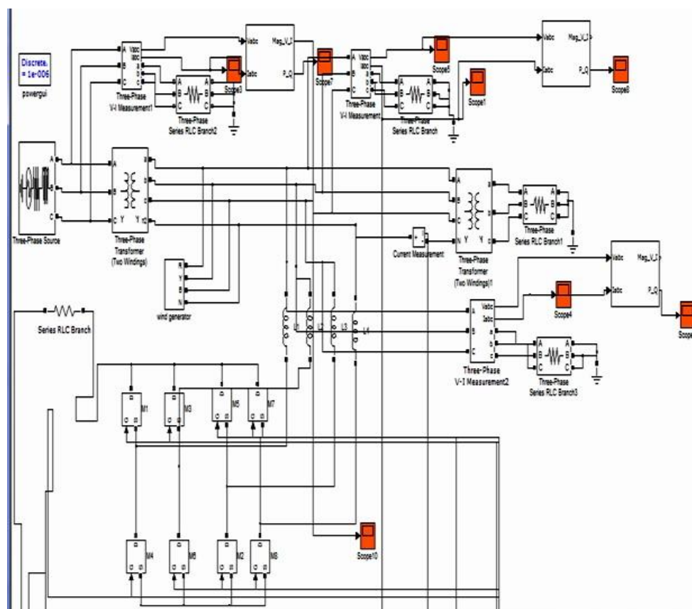
Fig 7 MATLAB Model of base circuit
