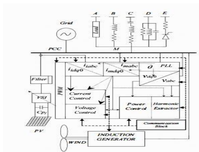
Fig 1 Functional Block Diagram of Proposed Model
