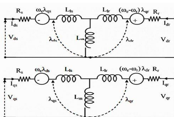
Fig.2-Equivalent circuit of IG - d-q model (a) d-axis
