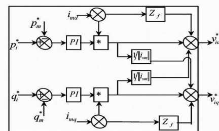
Fig 6. Proposed power control loops.
