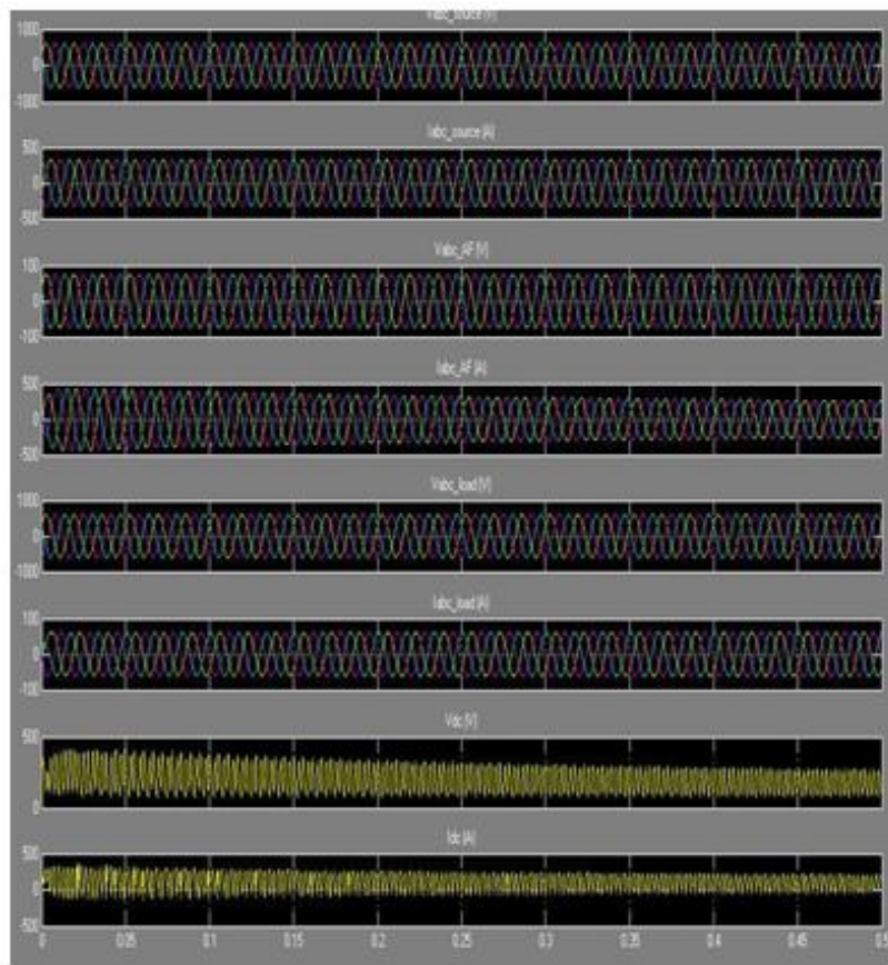
Fig.9 Wave form of voltage and current
