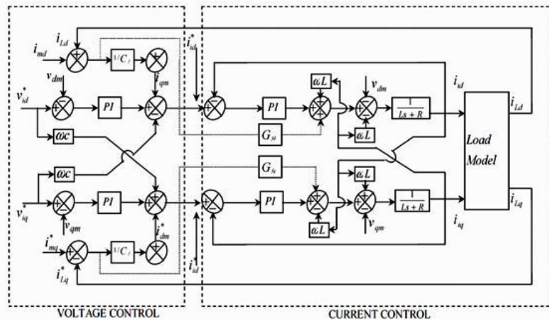
Fig3. Voltage control current control
