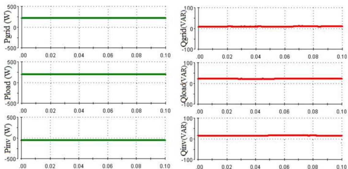
Fig. 7. Experimental results for the active power filtering mode : active and reactive power flow in real-time
