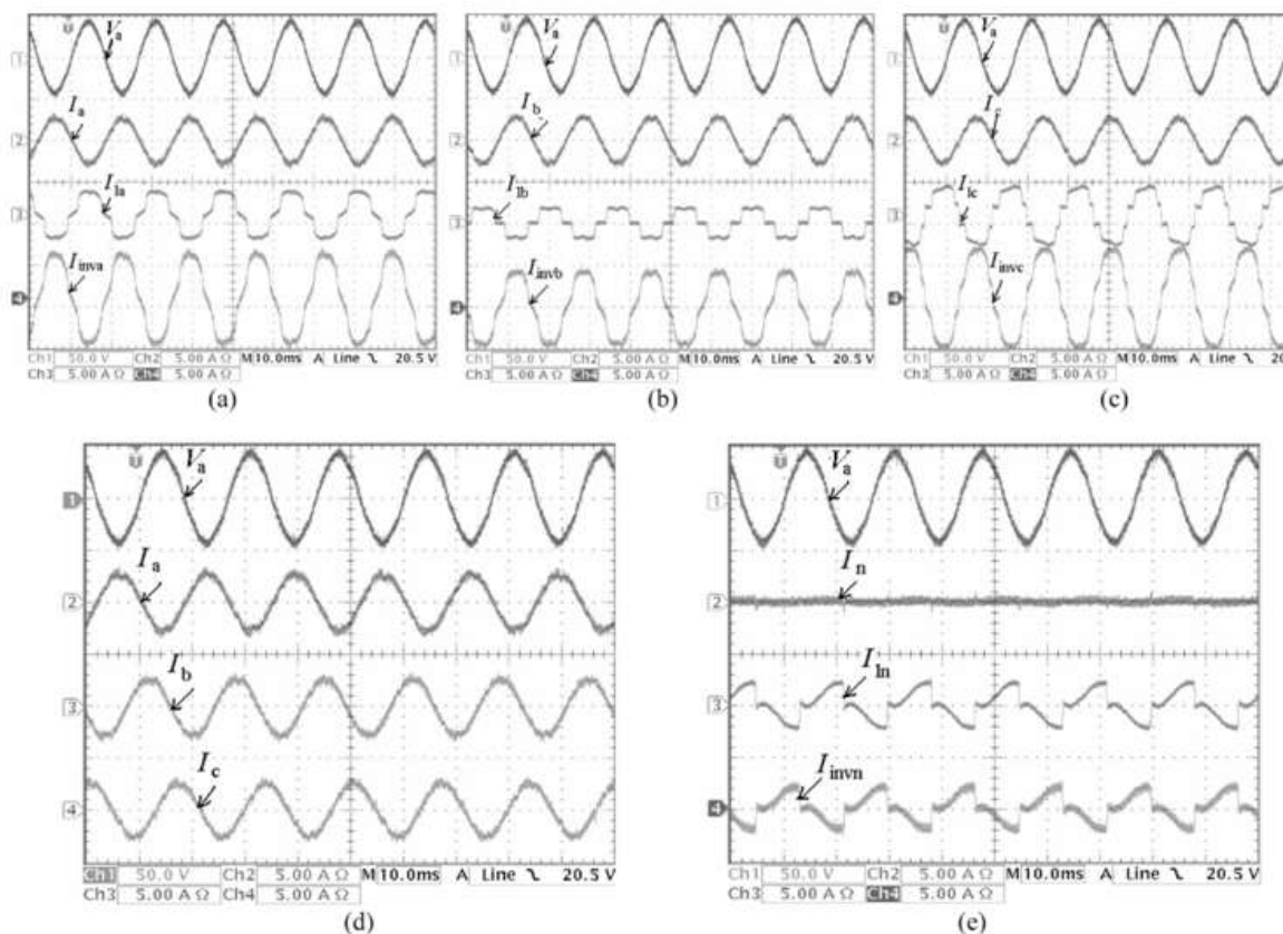
Fig. 8. Experimental results for the active power filtering and renewable power injection mode ( P_{RES} > P_L ): (a) phase a performance, (b) phase performance, (c) phase performance, (d) grid currents (e) load, grid and inverter neutral currents.
