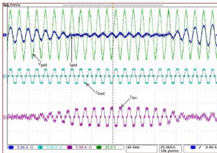
Fig. 10. Experimental results: Dynamic performance of proposed approach.
