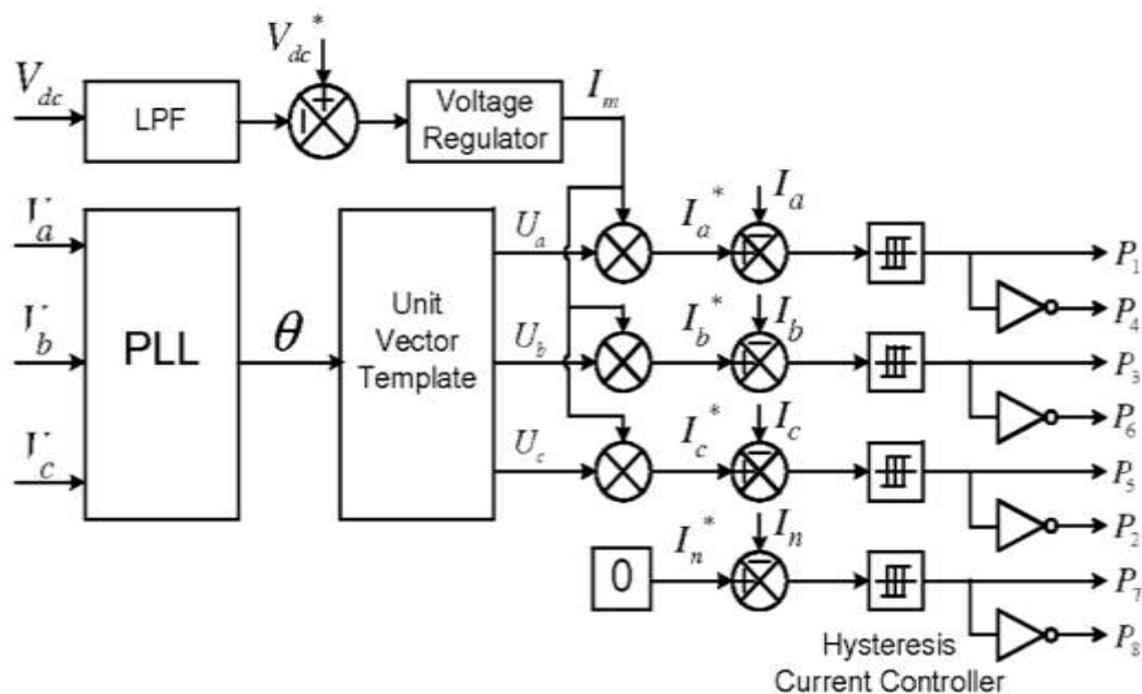
Fig. 3. Block diagram representation of grid-interfacing inverter control.
