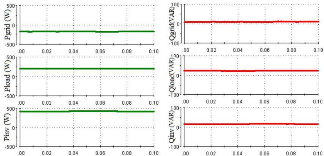
Fig. 9. Experimental results for the active power filtering and renewable power injection mode : active and reactive power flow in real time.
