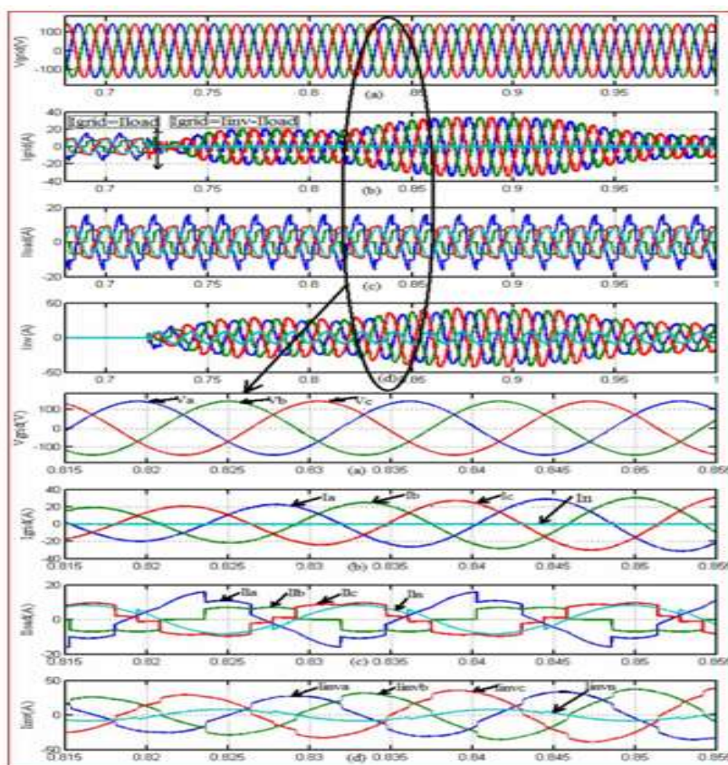
Fig. 4. Simulation results: (a) Grid voltages, (b) Grid Currents (c) Unbalanced load currents, (d) Inverter Currents.
