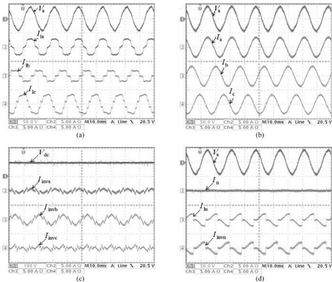
Fig. 6. Experimental results for the active power filtering mode : (a) unbalanced load currents, (b) grid currents after compensation, (c) currents injected by grid-interfacing inverter, (d) load, grid and inverter neutral currents.
