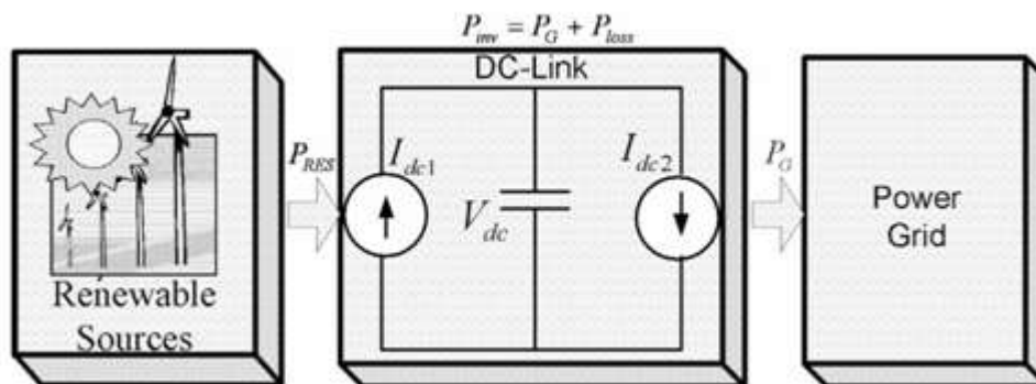
Fig. 2. DC-Link equivalent diagram.
