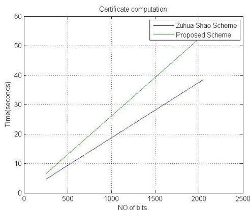
Graph1: Computation time (Seconds) of certificate calculation in Zuhua Shao scheme and proposed scheme
