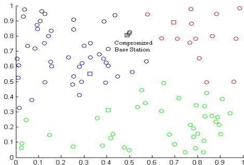
Figure 6. Improved LEAP protocol: A compromised base station
