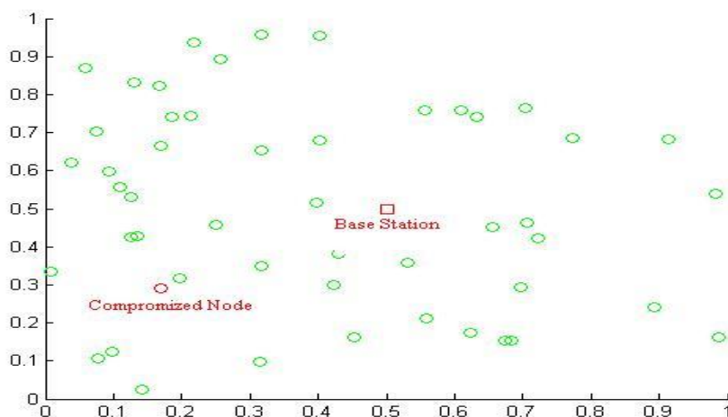
Figure 4. LEAP protocol: A compromised Sensor Node
