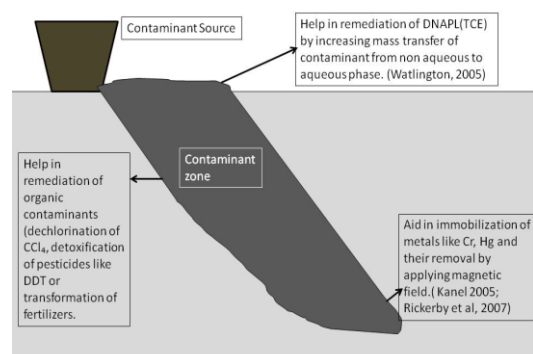
Figure 2. Schematic diagram representing the use of iron nanoparticles in the degradation of various environmental contaminants like organic, inorganic and petrochemical compounds.
