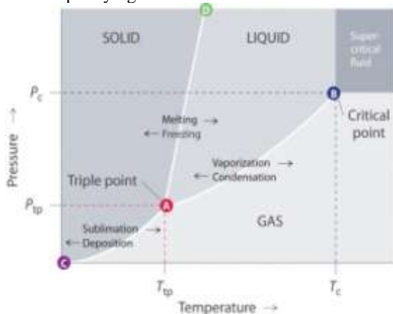
Figure shows phase diagram depicting the triple point A. The direct transition from solid to gas takes place along curve CA.
