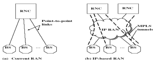
Fig. 2: Wireless access network architectures
