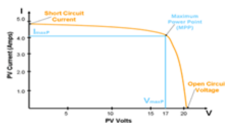
Fig.2: I-V characteristic curve of the cell
