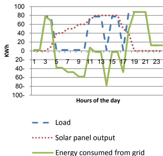
Fig.10: Solar system output, load and net energy consumed from grid
