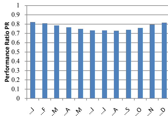
Fig.9 Performance Ratio.
