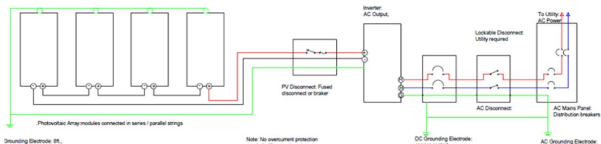
Fig.4 Grid-connected solar system
