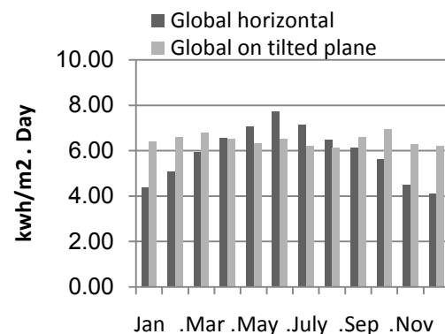
Fig.6 Meteo and incident energy from pvsyst software
