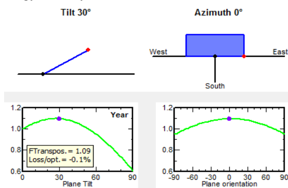
Fig.5: Tilt and Azimuth angles
