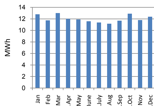
Fig.7 System output from pvsyst software
