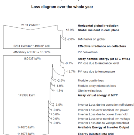
Fig.8: Loss diagram of the system over the year
