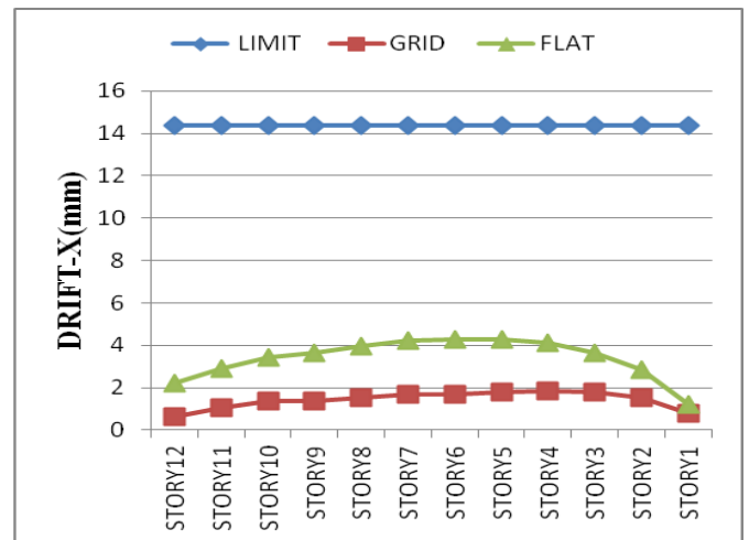
Graph 5 Comparison of building drift-X, zone II soil-2
