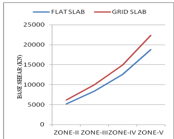
Graph 1 Seismic base shear in x-direction for soiltype-2
