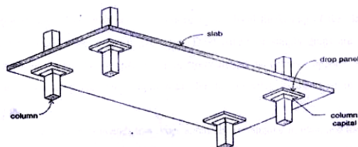
Figure-Flat slab system
