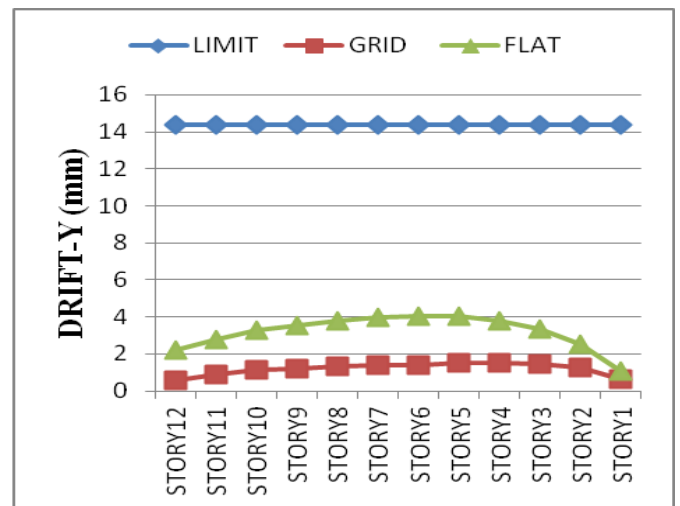
Graph 6 Comparison of building drift-Y, zone II soil-2
