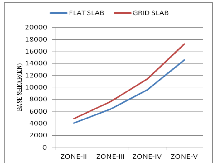
Graph 2 Seismic base shear in Y-direction for soiltype-2
