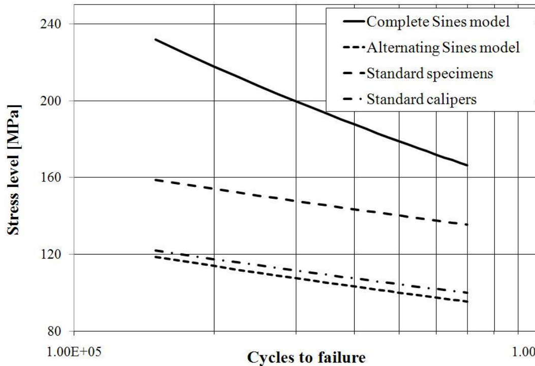
Fig. 10. Stress level vs. cycles to failure diagram: comparison between the predictions with the Sines criterion and the experimental data.
