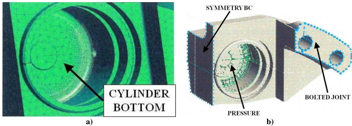
Fig. 8. (a) Mesh refinement at the bottom of the oil cylinder. (b) Loads and boundary conditions.
