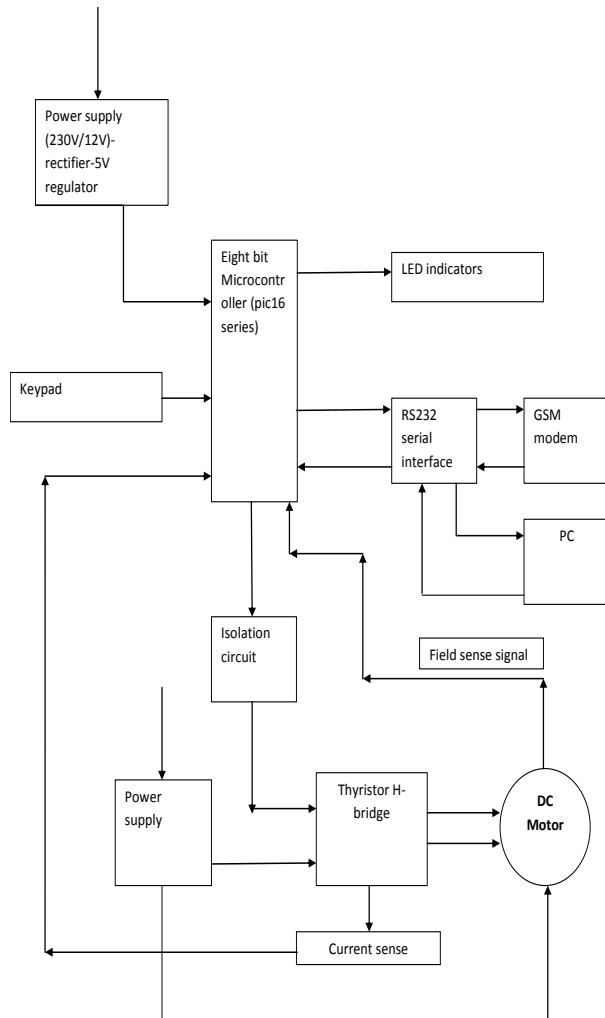
Fig.1 block diagram of the system
