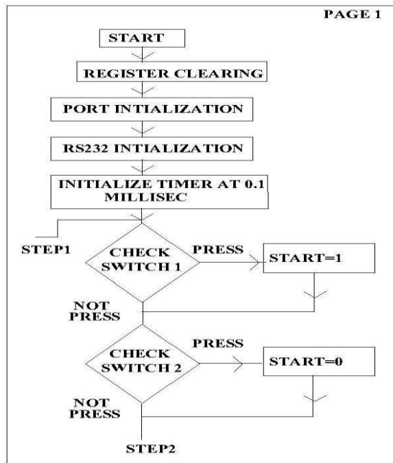
Fig.3 Flow chart 1 Algorithm For Manual Mode
