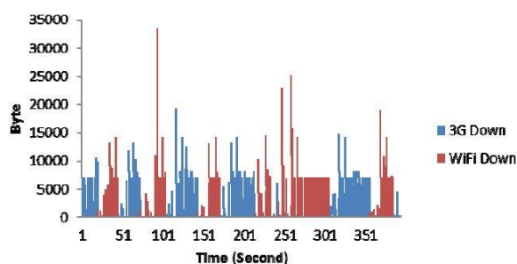
Figure 1. Received traffic with Android Wi-Fi connection manager
