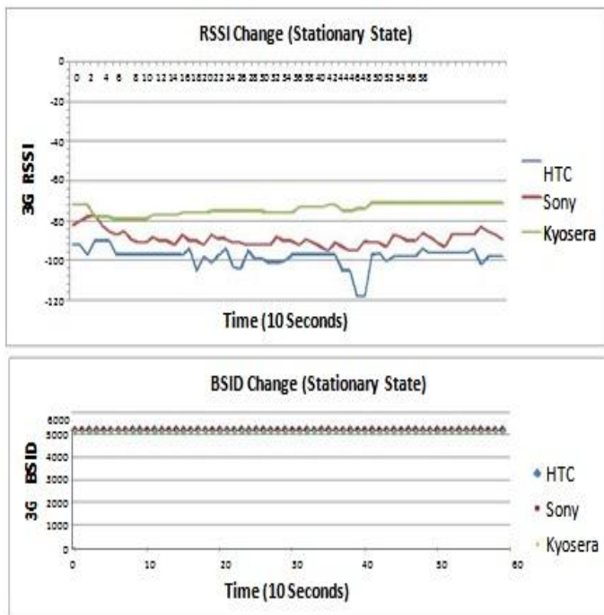
Figure 6. 3G RSSI/BSID Variation of Stationary State
