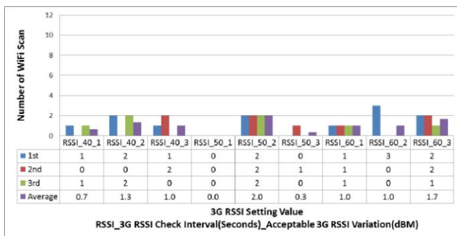
Figure 12. Number of Wi-Fi scan test results (3G RSSI check interval from 40 to 60 seconds)
