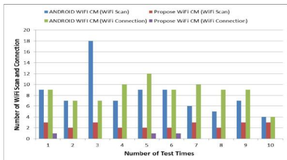
Figure 14. Comparison of a number of Wi-Fi scans and connections
