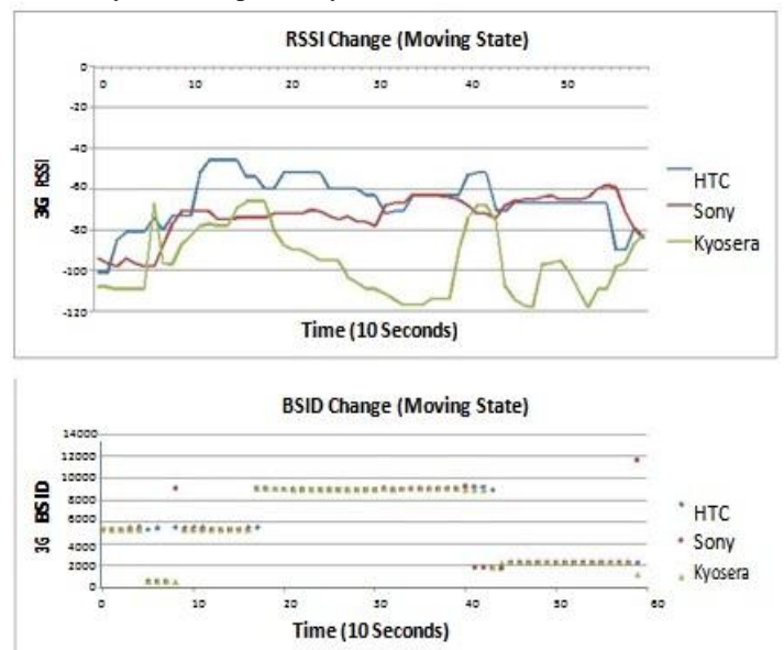
Figure 5. 3G RSSI/BSID Variation of Moving State
