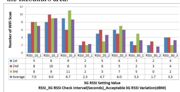
Figure 11. Number of Wi-Fi scan test results (3G RSSI check interval from 10 to 30 seconds)
