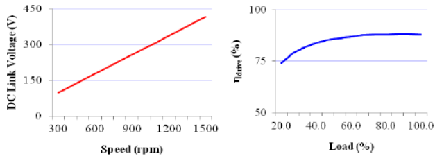
Fig.6a.DC link voltage with speed Fig.6b. Efficiency with load
