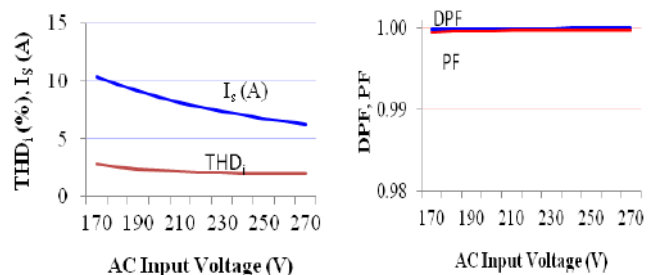
Fig. 9a. Current at AC mains and its THD Fig. 9b. DPF and PF
