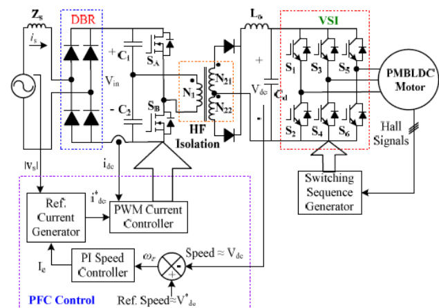
Figure 1. Control schematic of Proposed Bridge-buck PFC converter fed PMBLDCM drive
