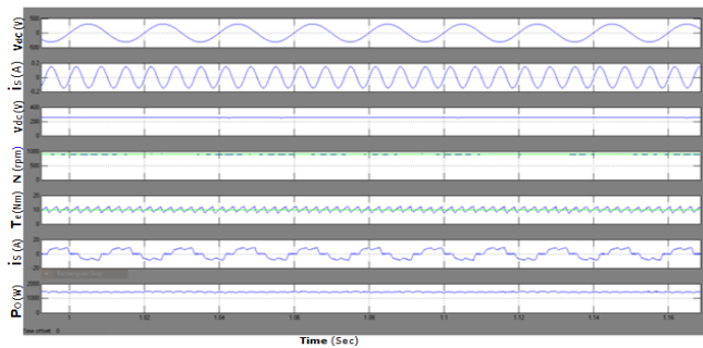
Fig: 4a Starting performance of the PMBLDCM drive at 900 rpm
