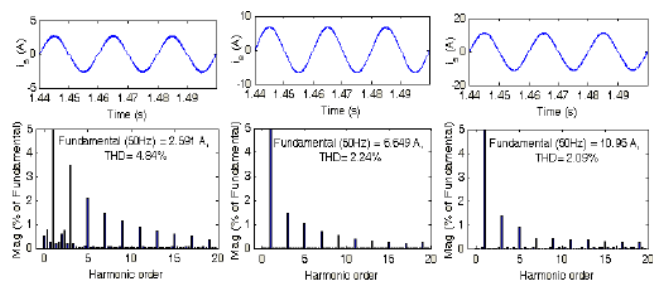
Fig. 8a. At 300 rpm Fig. 8b. At 900 rpm Fig. 8c. At 1500 rpm
