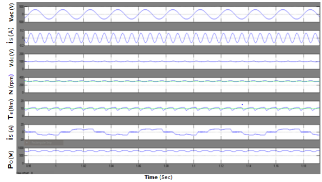
Fig: 5a Performance of the PMBLDCM drive at 300 rpm
