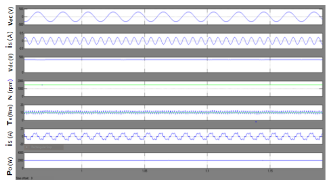
Fig: 5c Performance of the PMBLDCM drive at 1500 rpm
