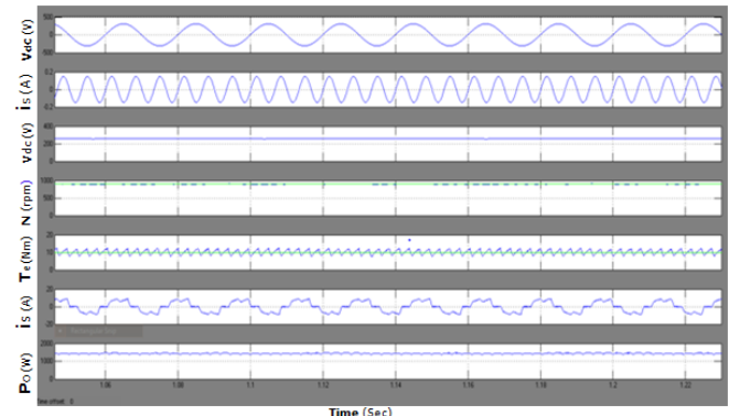
Fig: 5b Performance of the PMBLDCM drive at 900 rpm
