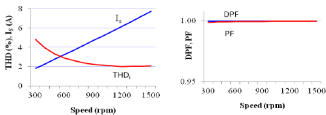
Fig.7a. THD of current at AC mains Fig. 7b. DPF and PF
