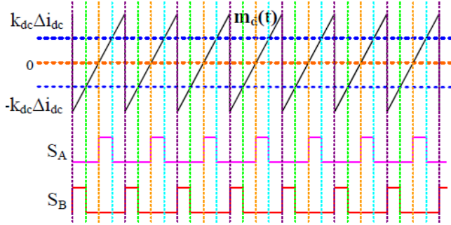
Figure 2. PWM control of the buck half-bridge converter
