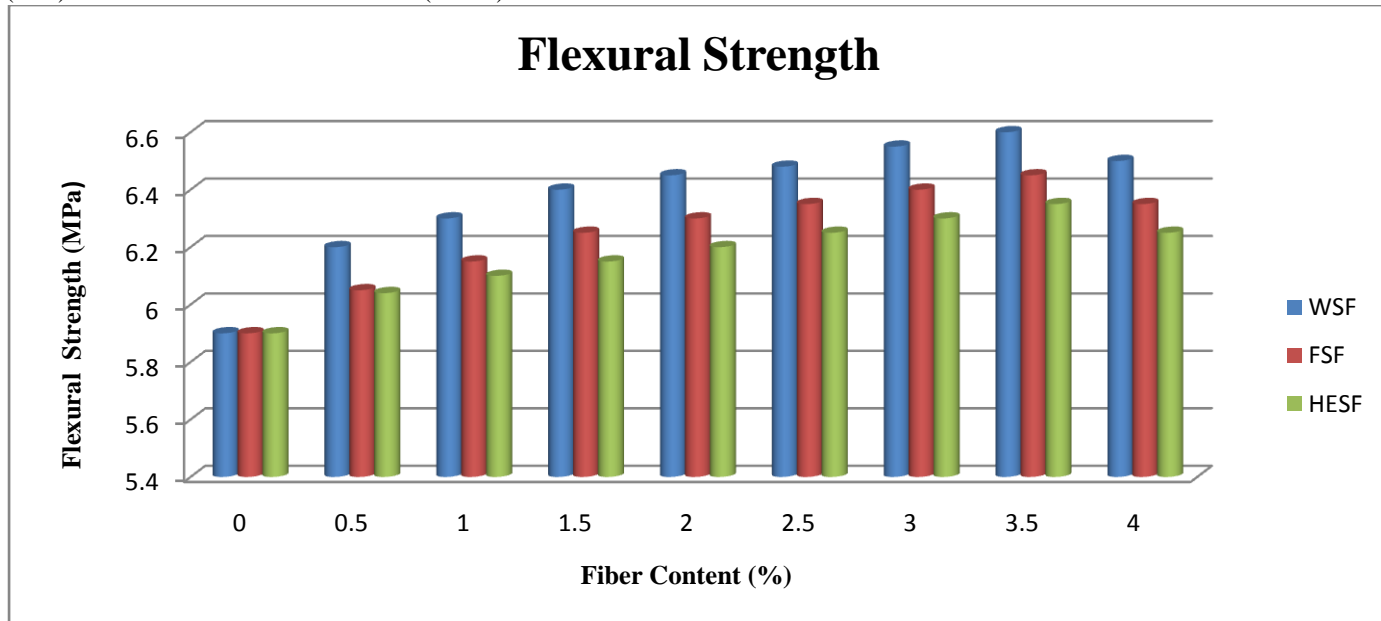
Fig. 5.1 Flexural Strength of concrete with percentage variation of Steel Fibres
