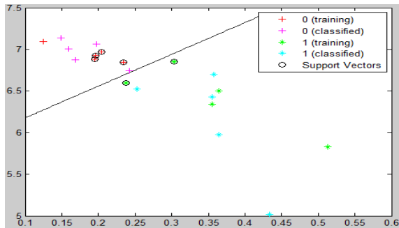
Fig:8 The classification using SVM
