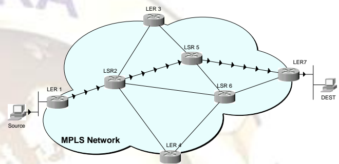
Figure 1 : MPLS Network
