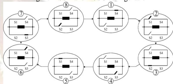
Fig. 2. Switching status of the VCB configuration.
