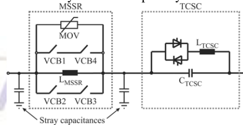
Fig. 1. MSSR and TCSC configuration
