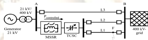
Fig. 3. MSSR and TCSC—Electric network configuration.
