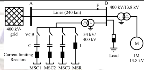
Fig. 4. MSD—Electric network configuration
