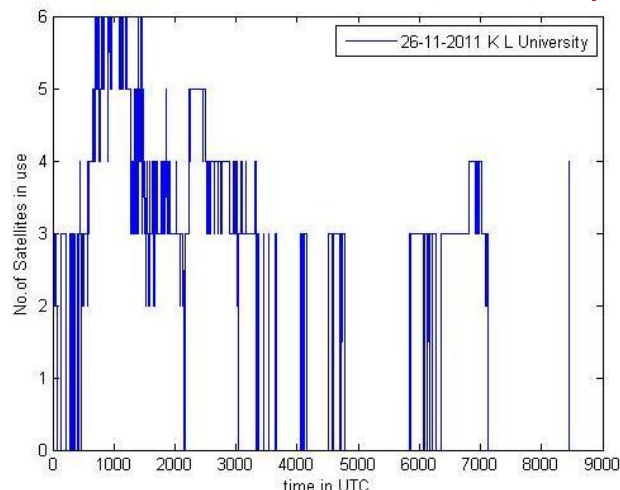
Figure 5: Number of visible satellites
