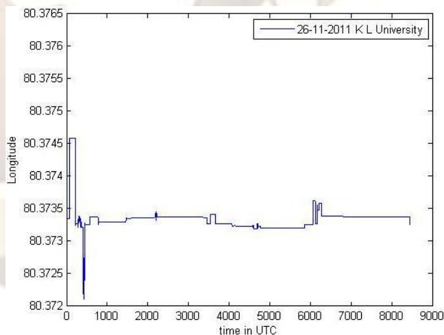
Figure 4: Longitudinal positional variations using single frequency GPS receiver
