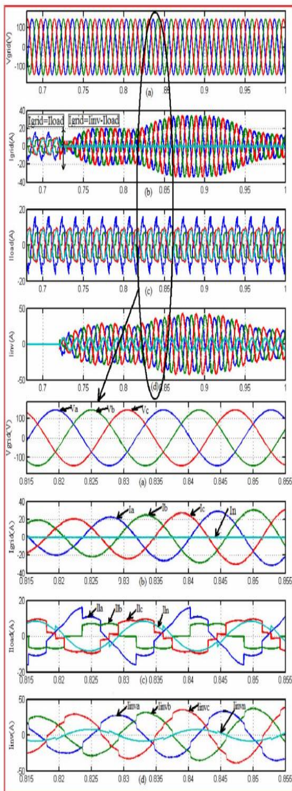
Fig. 4. Simulation results: (a) Grid voltages, (b) Grid Currents (c) Unbalanced load currents, (d) Inverter Currents
