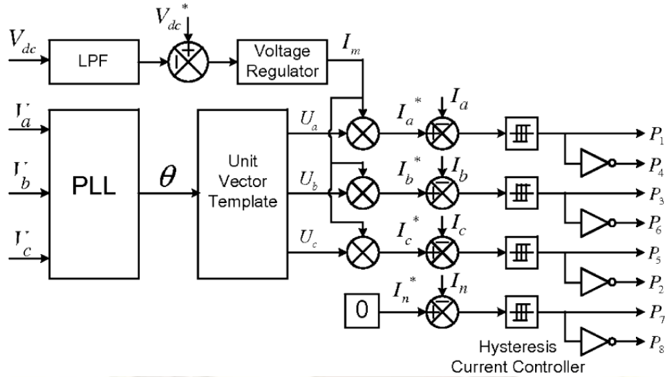
Fig. 3. Block diagram representation of grid-interfacing inverter control
