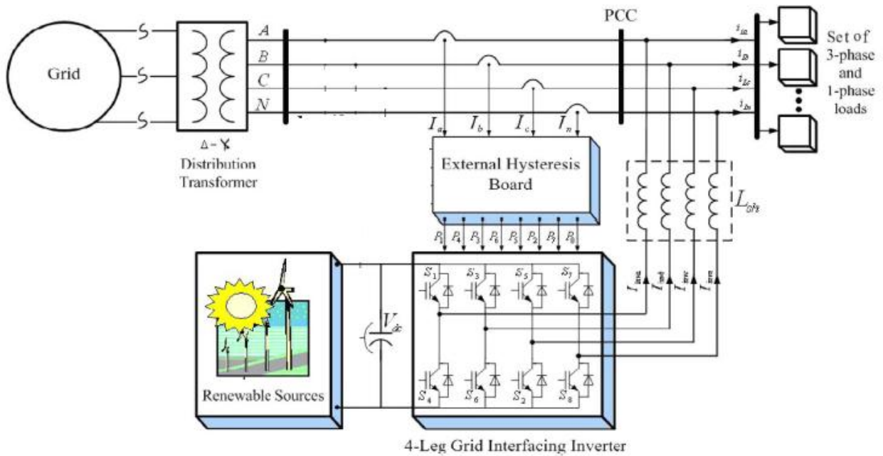
4-Leg Grid Interface Inverter Fig. 1. Schematic of proposed renewable based distributed generation system
