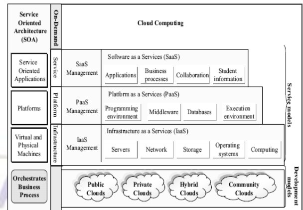
Figure 2.1 Relationship between SOA and Cloud Computing
