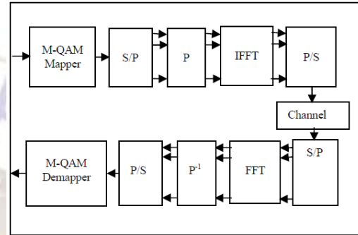
Fig. 2. Block diagram of Pre IFFT based OFDM system The Precoding matrix P can be written as
