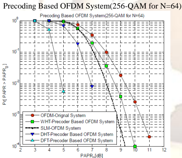
Fig.6. CCDF comparison of DHT-Precoder Based OFDM System with DFT-Precoder Based OFDM system, WHT-Precoder Based OFDM System, SLM-OFDM (V=2) System and OFDM Original System for 256-QAM
