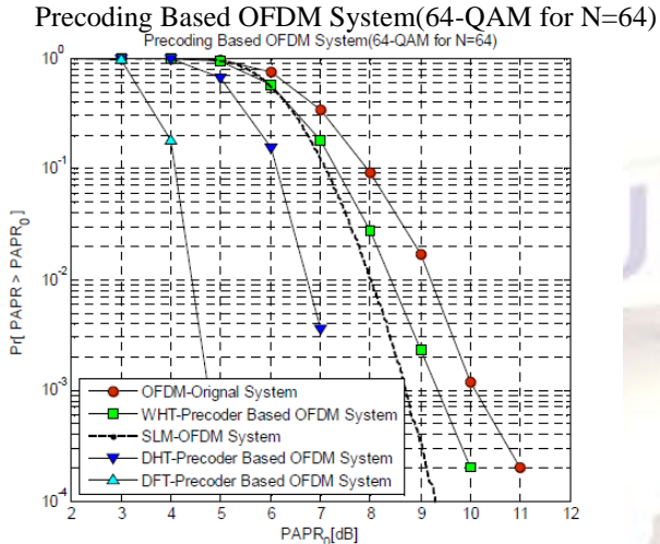
Fig.5. CCDF comparison of DHT-Precoder Based OFDM System with DFT-Precoder Based OFDM system, WHT-Precoder Based OFDM System, SLM-OFDM (V=2) System and OFDM Original System for 64-QAM
