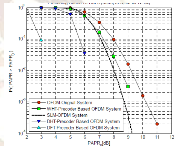
Figure.3. CCDF comparison of DHT-Precoder Based OFDM System with DFT-Precoder Based OFDM system, WHT-Precoder Based OFDM System, SLM-OFDM (V=2) System and OFDM Original System for 16-QAM
