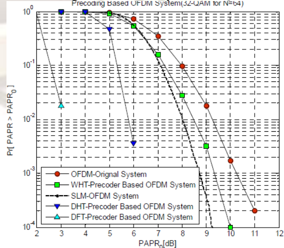
Precoding Based OFDM System(32-QAM for N=64)
