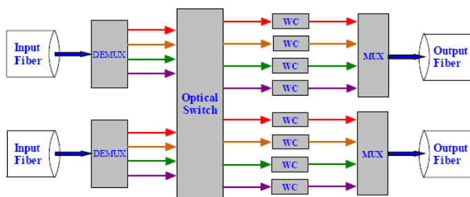
Fig:5 wavelength converter with fullwavelength conversion
