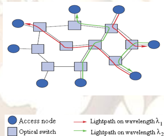
Fig 1: A wavelength routed optical WDM network with lightpath connections
