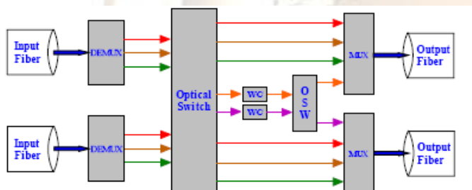
Fig:6 wavelength converter with partial wavelength conversion
